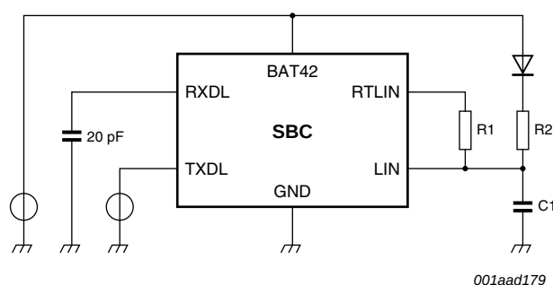
Fig 27. Timing test circuit for LIN transceiver
