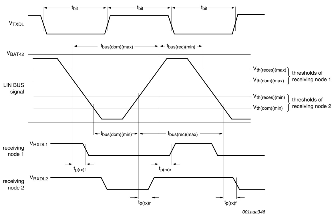
Fig 28. Timing diagram LIN transceiver
