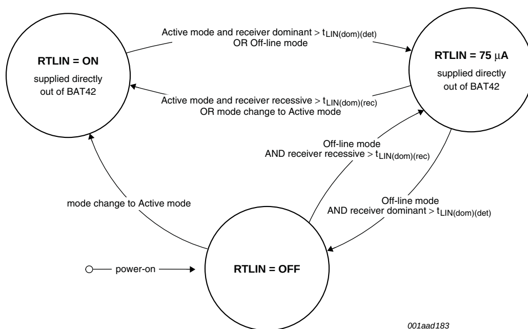
Fig 11. States of the RTLIN pin
