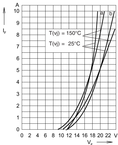
Fig. 1: Forward characteristics
