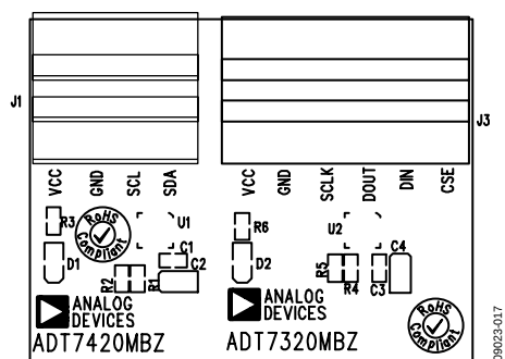
Figure 17. ADT7x20 Evaluation Board External Board Silkscreen
