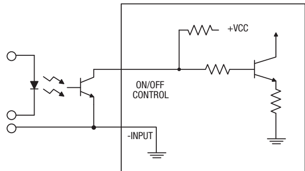
Figure 10. Driving the On/Off Control Pin (suggested circuit)
