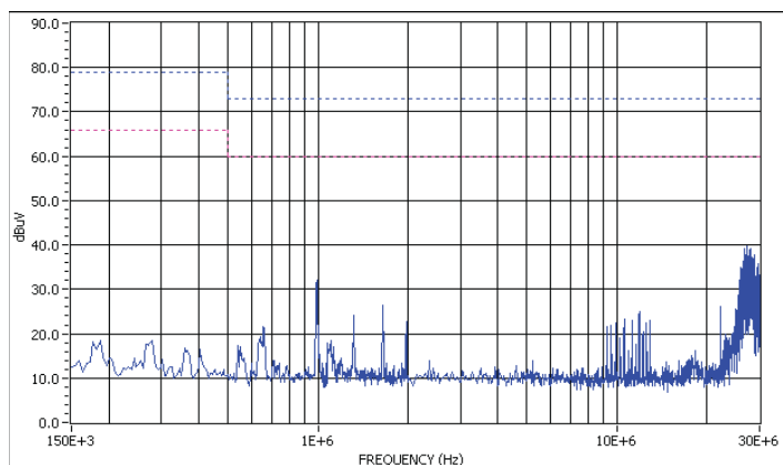
Graph 3. Conducted emissions performance, Positive Line, CISPR 22, Class A, full load
