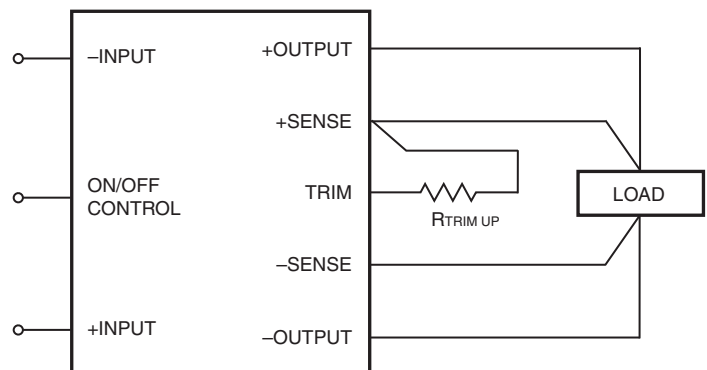
Figure 8. Trim Connections To Increase Output Voltages
