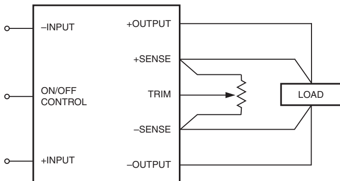
Figure 7. Trim Connections Using A Trimpot
