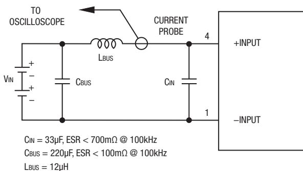
Figure 4. Measuring Input Ripple Current
