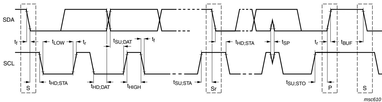
Fig 20. I 2 C-bus timing
