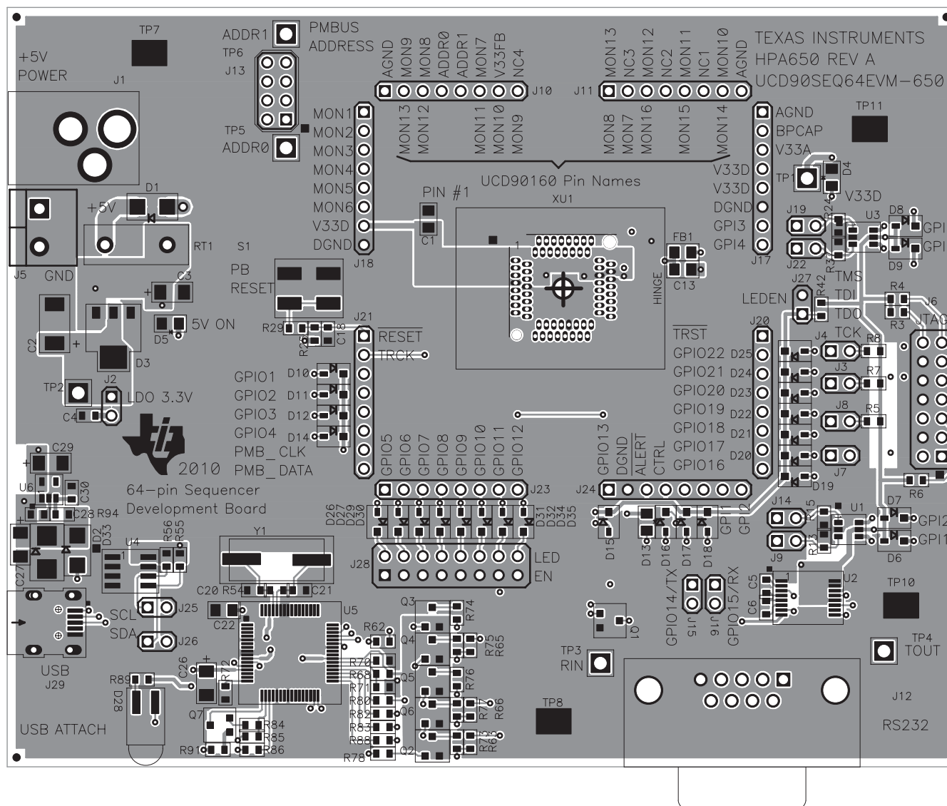
Figure 4. Top-Side Layout/Routing
