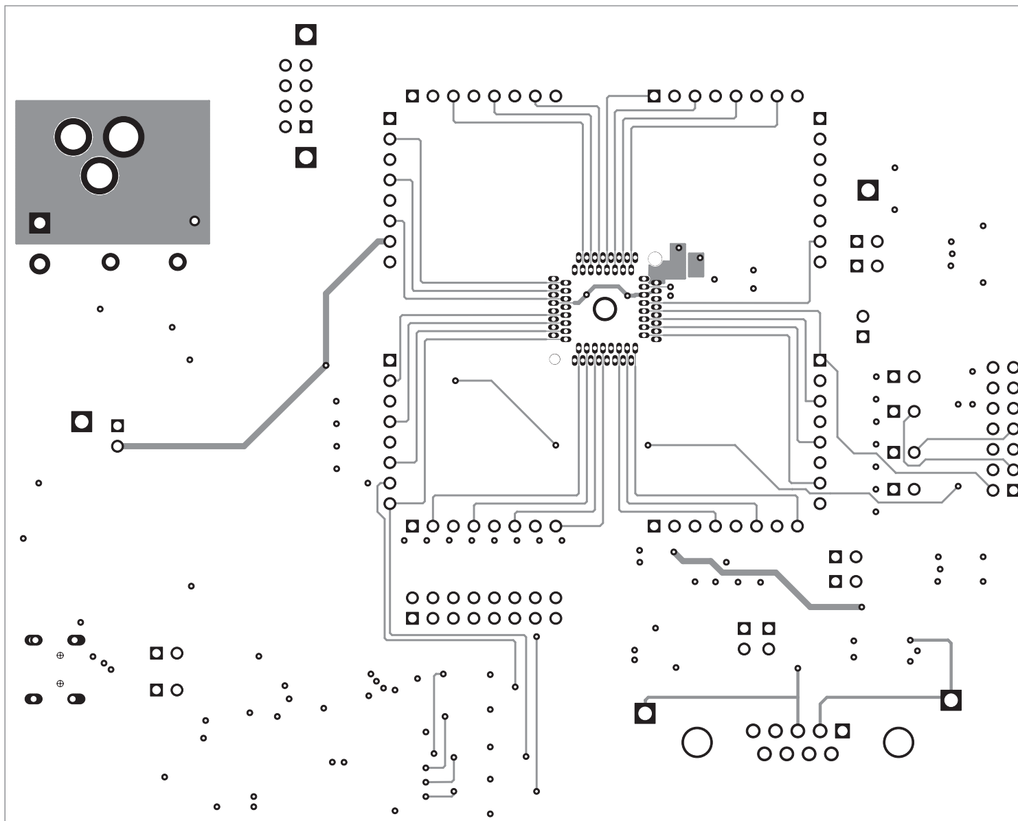
Figure 6. Layer-3 Routing
