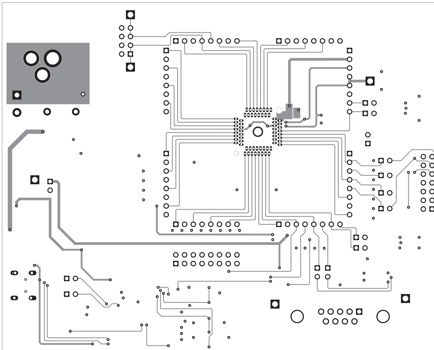
Figure 5. Layer-2 Routing
