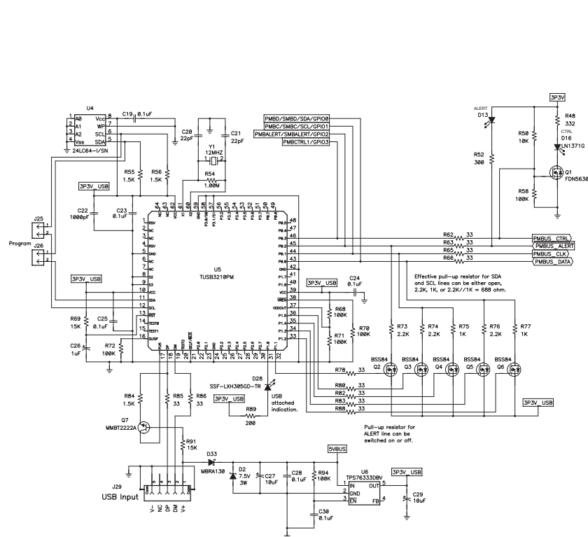
Figure 3. Figure 3. UCD90SEQ64EVM-650 Schematic (sheet 2 of 2)
