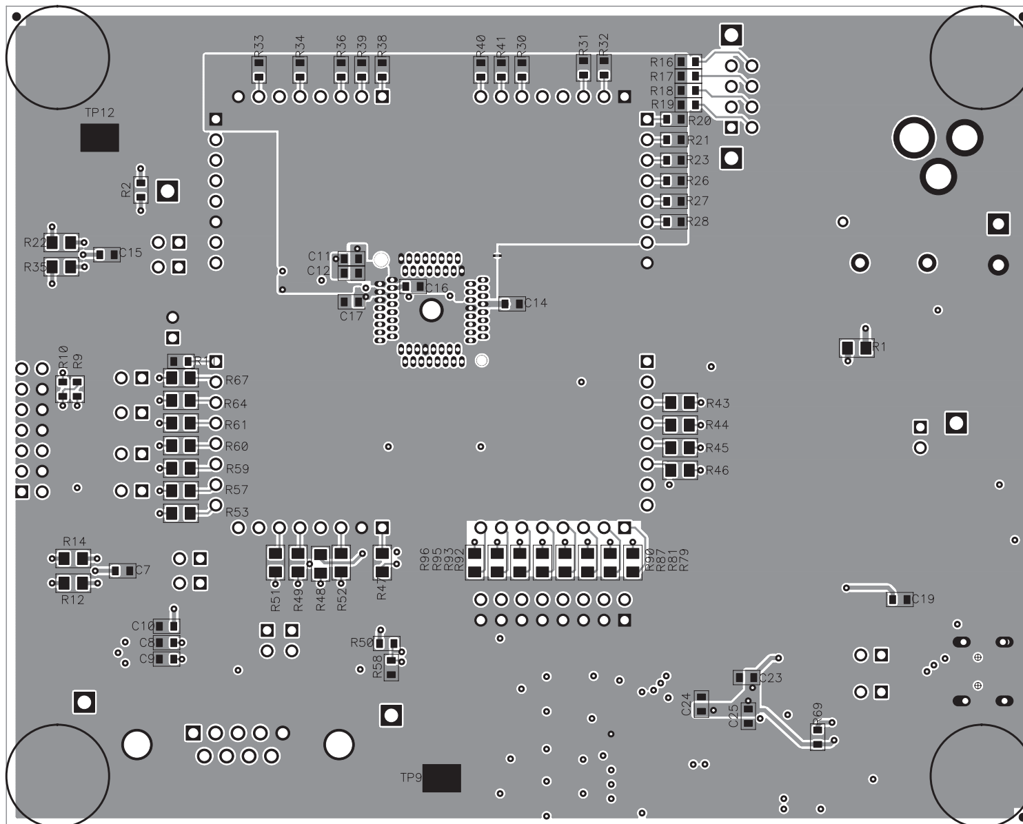
Figure 7. Bottom-Side Placement/Routing
