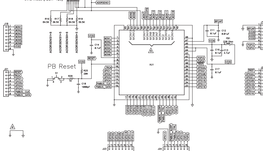
Figure 2. UCD90SEQ64EVM-650 Schematic (Sheet 1 of 2)
