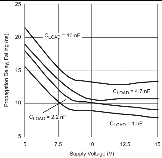
Figure 16. CLK to OUTx Propagation Delay Falling vs Supply Current
