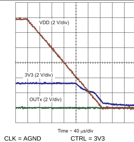
Figure 24. Shut-Down Behavior at V_{DD} = 12\text{ V}
