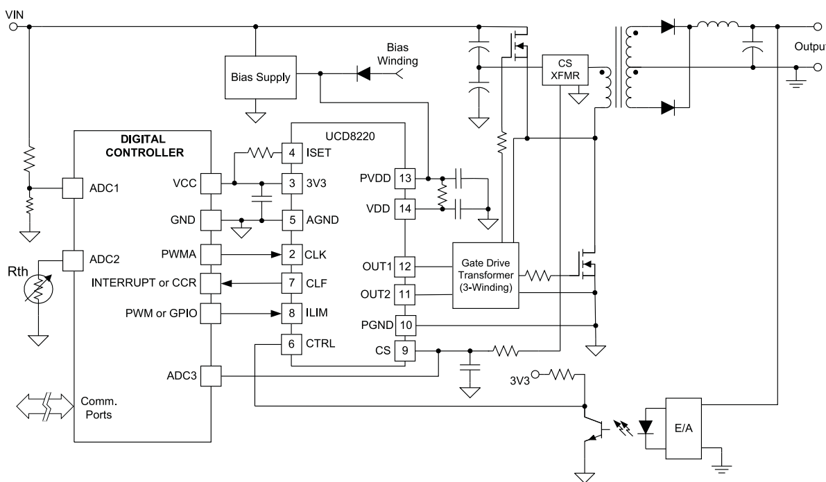
Figure 31. UCD8220 Typical Simplified Half-Bridge Converter Application Schematic
