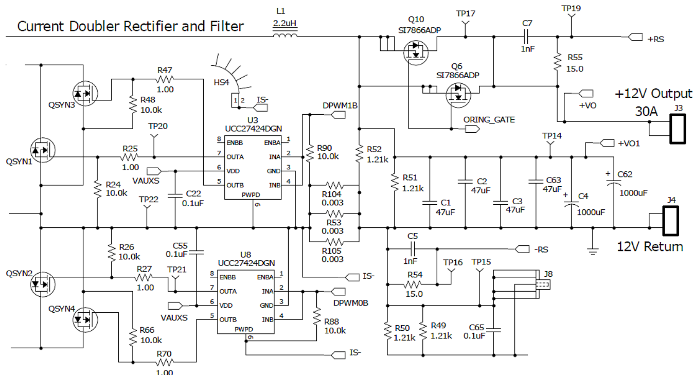
Figure 26. Load-Current Sensing Connections
