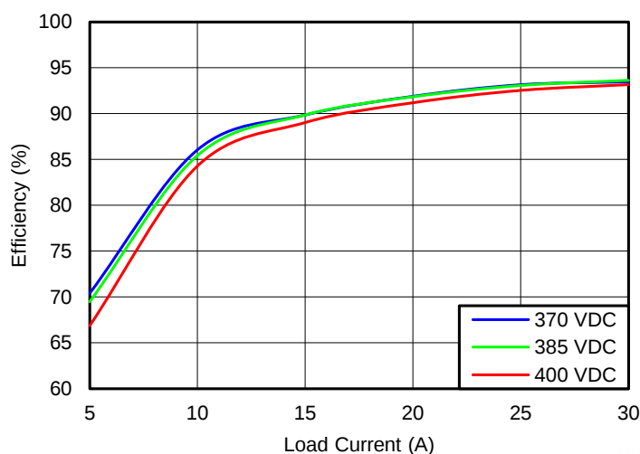
Figure 7. UCD3138PSFBEVM-027 Efficiency
