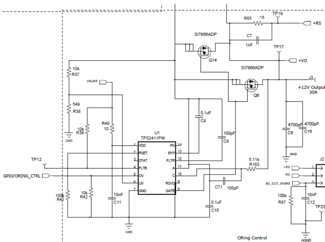
Figure 39. Oring Control
