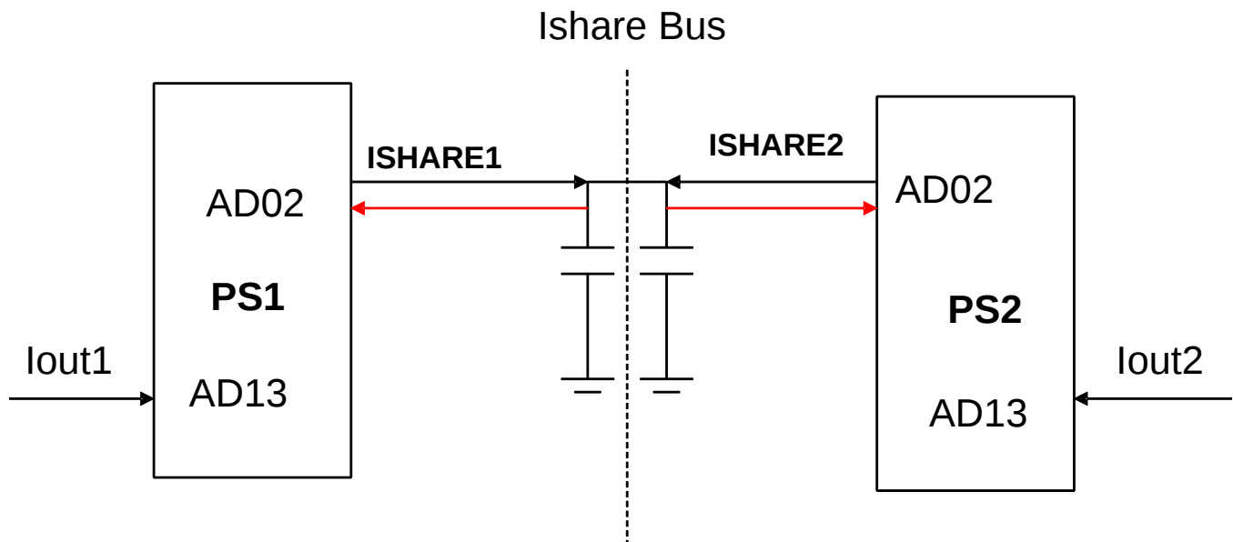
Figure 38. Current-Sharing Operation
