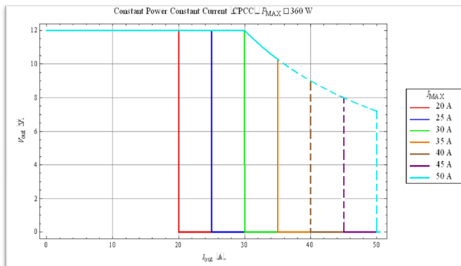
Figure 33. CCPCC Operation
