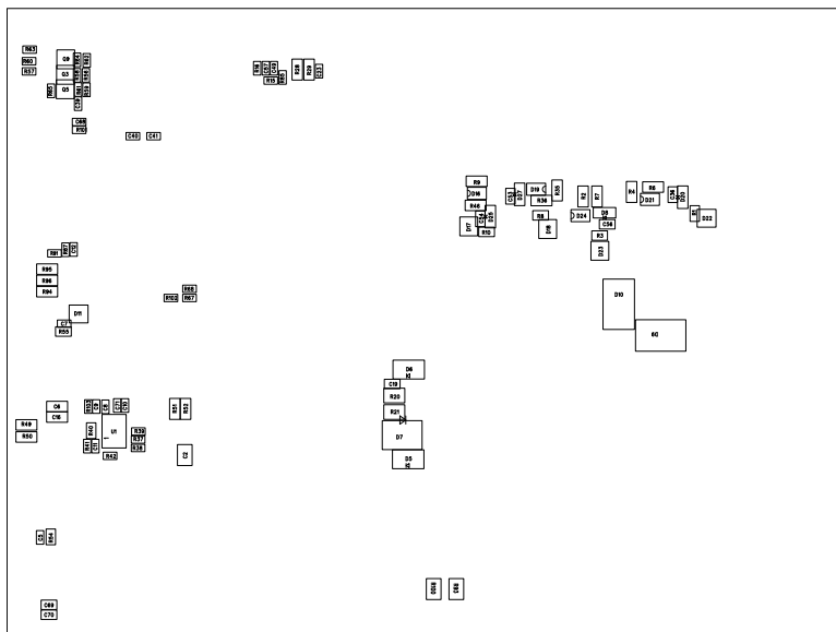
Figure 17. UCD3138PSFBEVM-027 Bottom-Layer Assembly Drawing (Bottom view)
