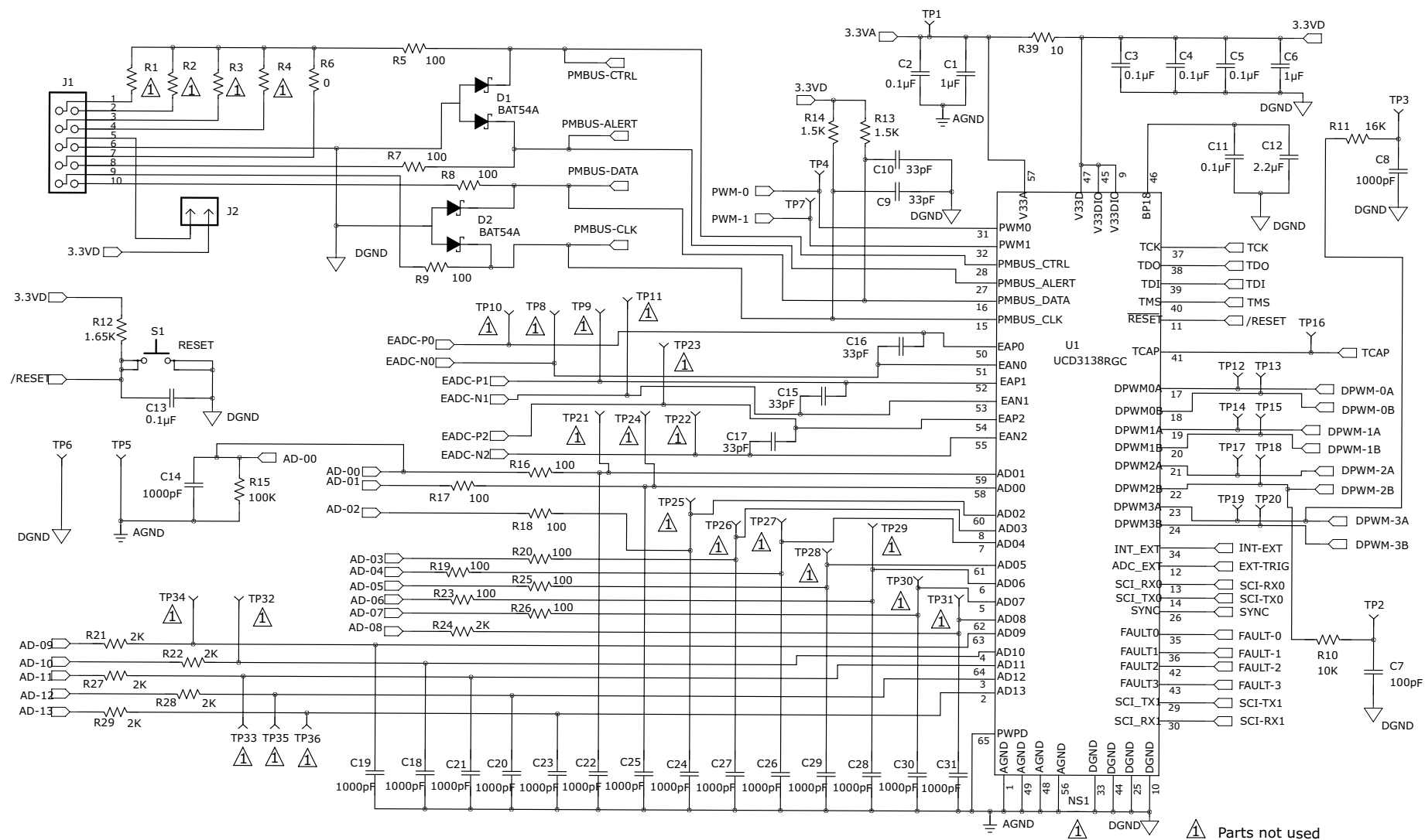
Figure 3. UCD3138CC64EVM-030 Schematics, Sheet 1 of 2
