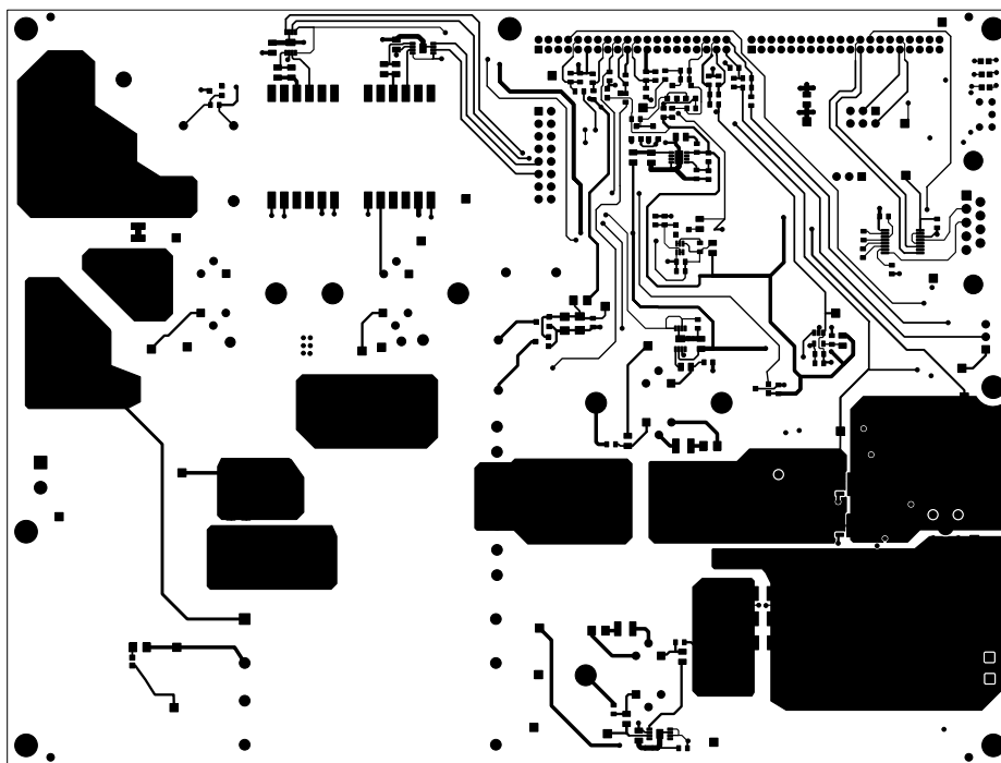
Figure 18. UCD3138PSFBEVM-027 Top Copper (Top View)
