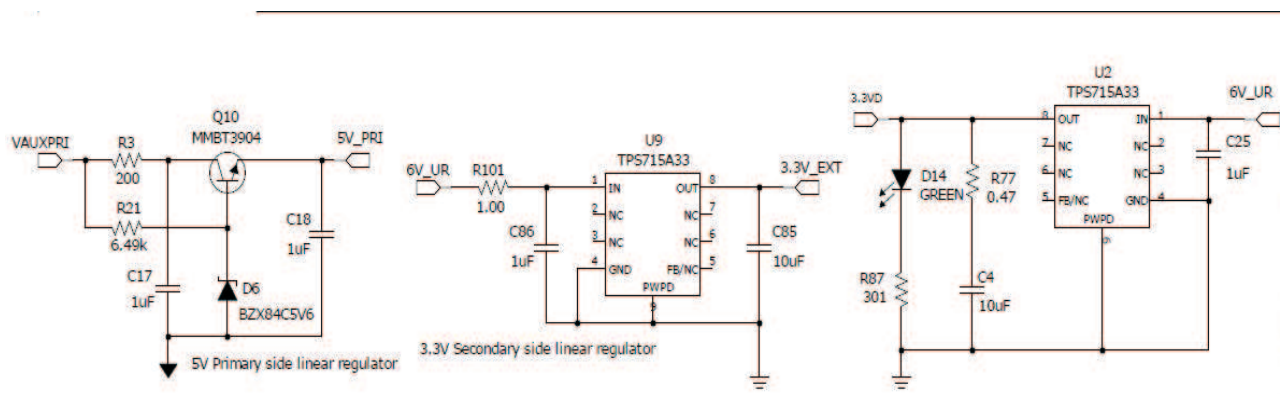
Figure 25. LDO Bias Circuits
