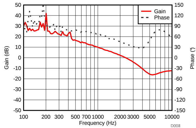
Figure 0-25. Control Loop Bode Plots at 400 V DC and Full Load
