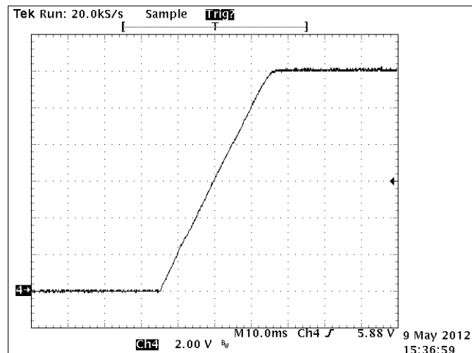
Figure 21. Output Turn On 380 V DC with Load Range
