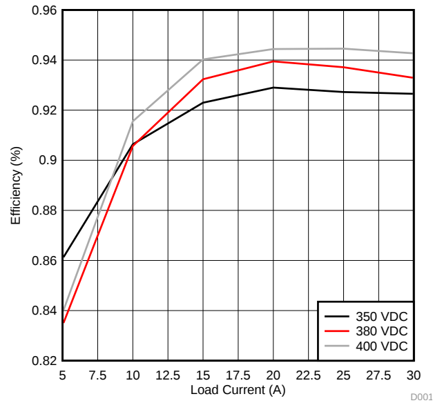
Figure 0-12. UCD3138ALLCEVM150 Efficiency
