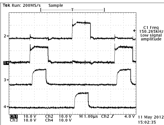
Figure 16. PWM Mode Operation after F_{SW} = 150 kHz (Ch1 = V_{GS} of Q7, Ch2 = V_{GS} of Q6, Ch3 = V_{GS} of SR2, Ch4 = V_{GS} of SR3)
