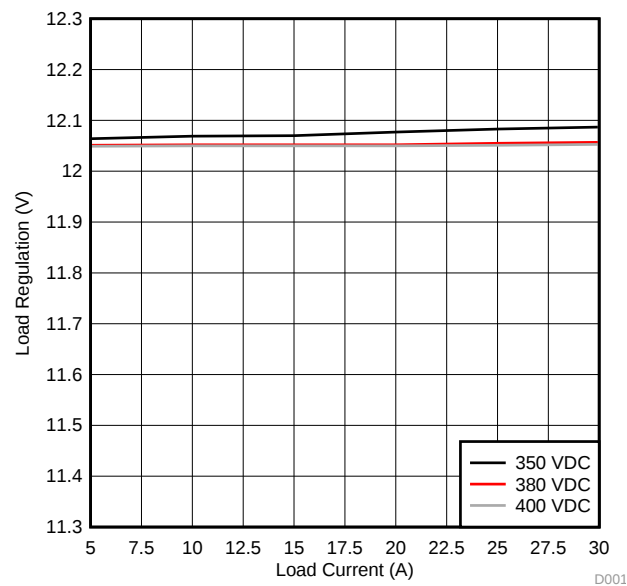
Figure 0-13. UCD3138ALLCEVM150 Load Regulation
