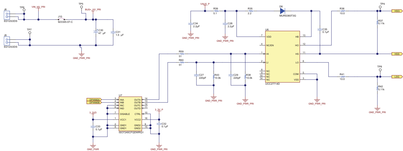
Figure 0-5. UCD3138ALLCEVM150 Schematics (5 of 9)
