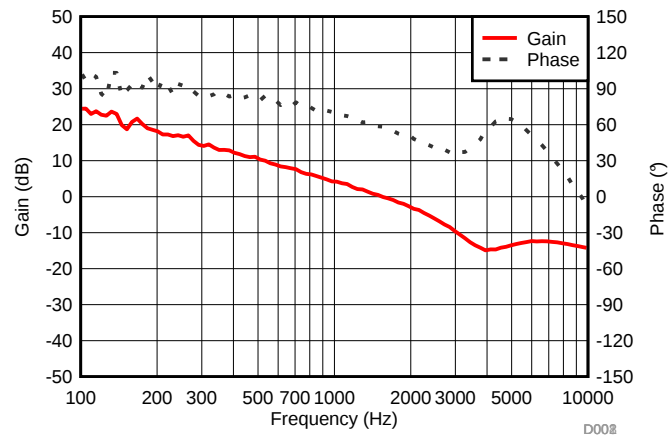
Figure 0-24. Control Loop Bode Plots at 380 V DC and Full Load
