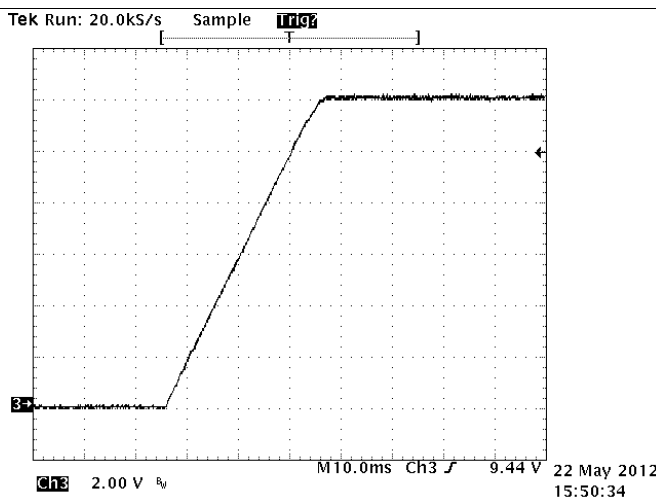
Figure 22. Output Turn On 350 V DC with Load Range
