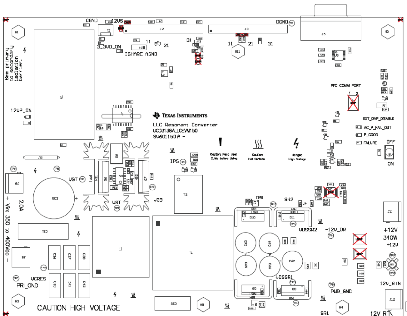
Figure 0-26. UCD3138ALLCEVM150 Top Layer Assembly Drawing (Top View)
