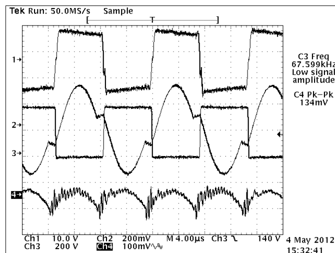
Figure 15. LLC Resonant Mode Operation at Full Load (Ch1 = V_{GS} of Q7, Ch2 = current in resonant network, 2 A/div, Ch3 = V_{DS} of Q7, Ch4 = V_O ripple)
