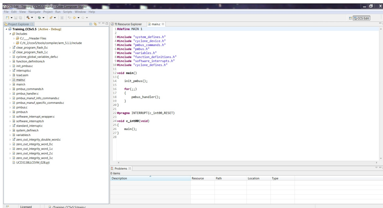
Figure 16. Project Explorer
