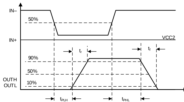
Figure 43. t_{PLH} and t_{PHL} Propagation Delay, Inverting Configuration
