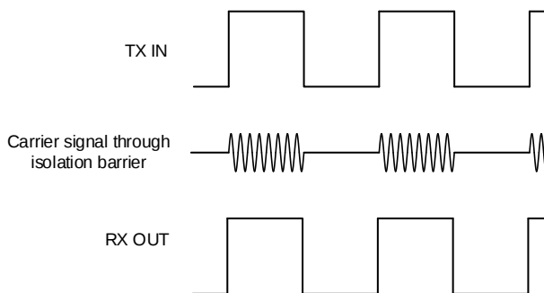
Figure 48. On-Off Keying (OOK) Based Modulation Scheme
