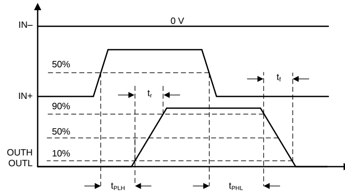
Figure 42. t_{PLH} and t_{PHL} Propagation Delay, Noninverting Configuration
