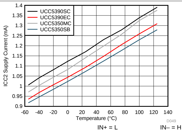
Figure 17. I_{CC2} Supply Current vs Temperature
