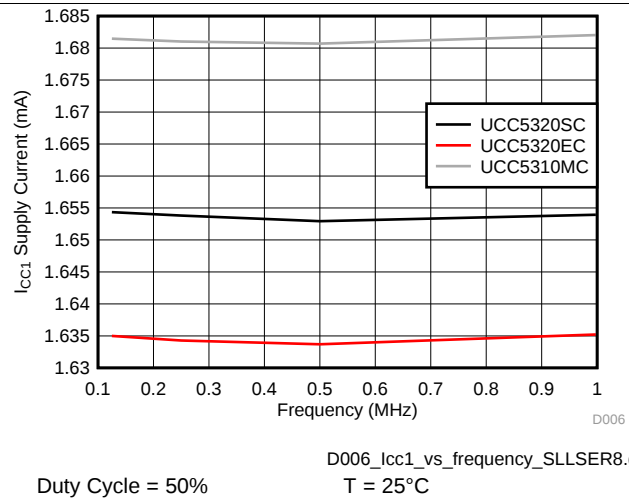
Figure 14. I_{CC1} Supply Current vs Input Frequency
