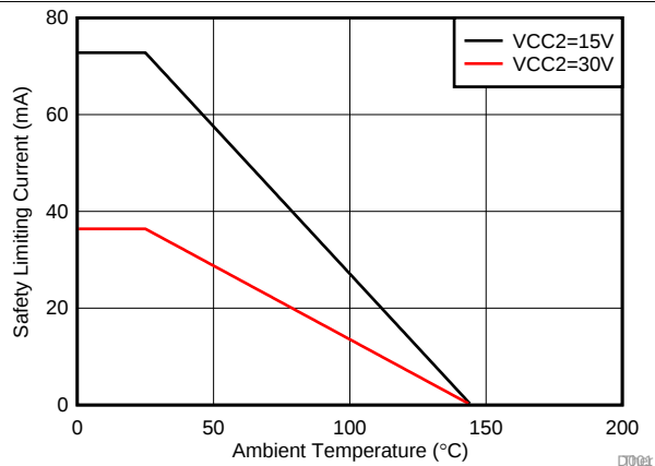
Figure 1. Thermal Derating Curve for Limiting Current per VDE for D Package
