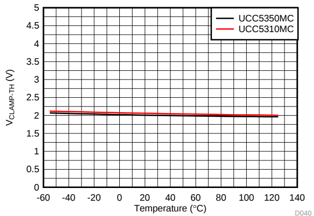
Figure 24. UCC5310M V_{CLAMP} vs Temperature
