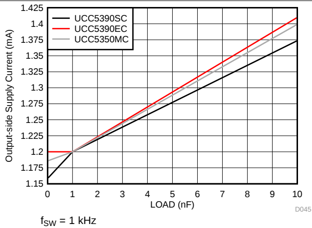
Figure 23. I_{CC2} Supply Current vs Load Capacitance
