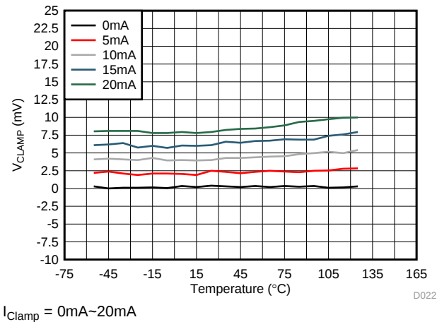
Figure 25. UCC5350M V_{CLAMP} vs Temperature
