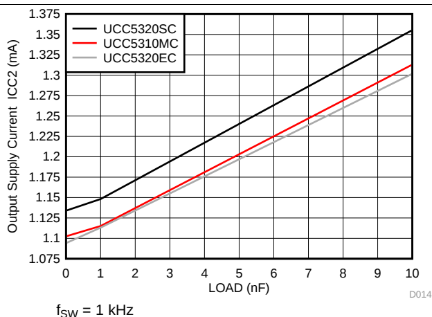
Figure 22. I_{CC2} Supply Current vs Load Capacitance
