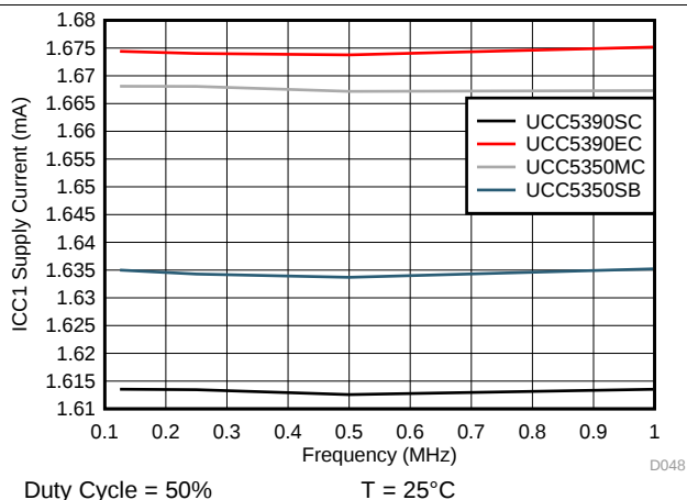
Figure 15. I_{CC1} Supply Current vs Input Frequency
