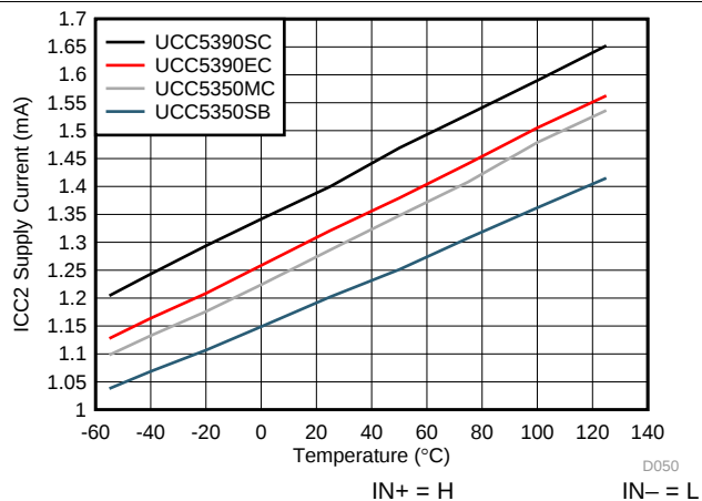
Figure 19. I_{CC2} Supply Current vs Temperature
