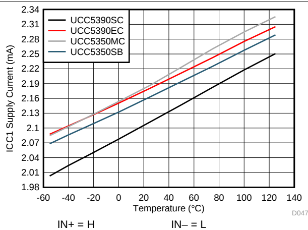
Figure 13. I_{CC1} Supply Current vs Temperature
