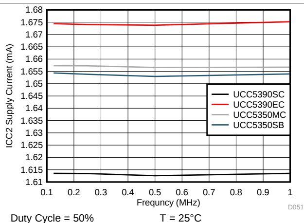
Figure 21. I_{CC2} Supply Current vs Input Frequency
