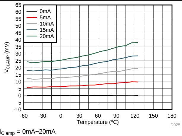
Figure 24. UCC5310M V_{CLAMP} vs Temperature
