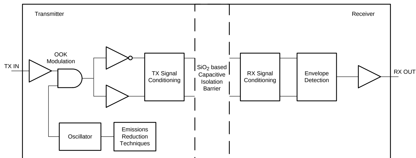
Figure 47. Conceptual Block Diagram of a Capacitive Data Channel
