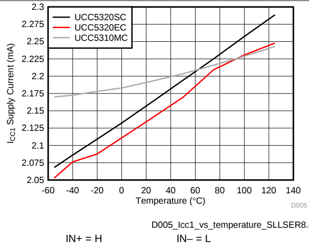
Figure 12. I_{CC1} Supply Current vs Temperature
