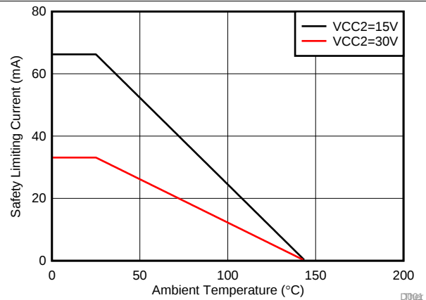
Figure 2. Thermal Derating Curve for Limiting Current per VDE for DWV Package
