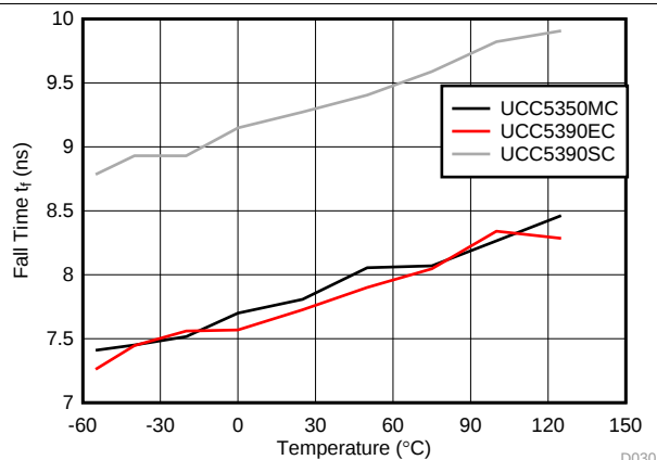
Figure 30. Fall Time vs Temperature
