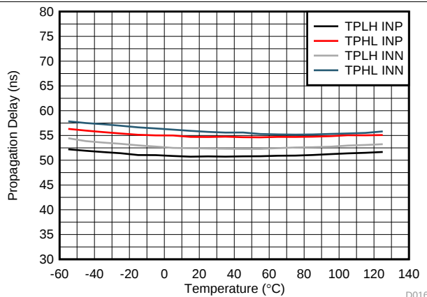
Figure 31. Propagation Delay t_{PLH} vs Temperature
