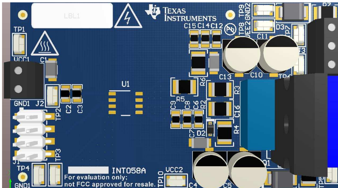
Figure 66. 3-D PCB View
