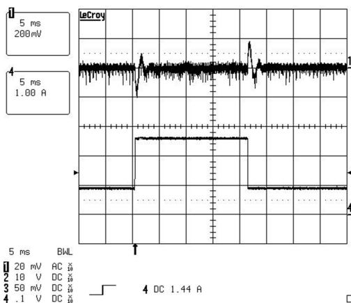
Figure 40. Output Voltage During 0.9-A to 2.7-A Load Transient (CH1: Output Voltage AC Coupled, 200 mV/div; CH4: Output Current, 1 A/div)
