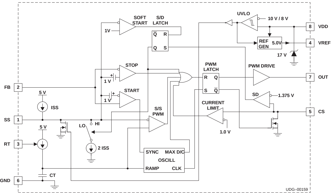
Figure 1. UCC3960 Block Diagram
