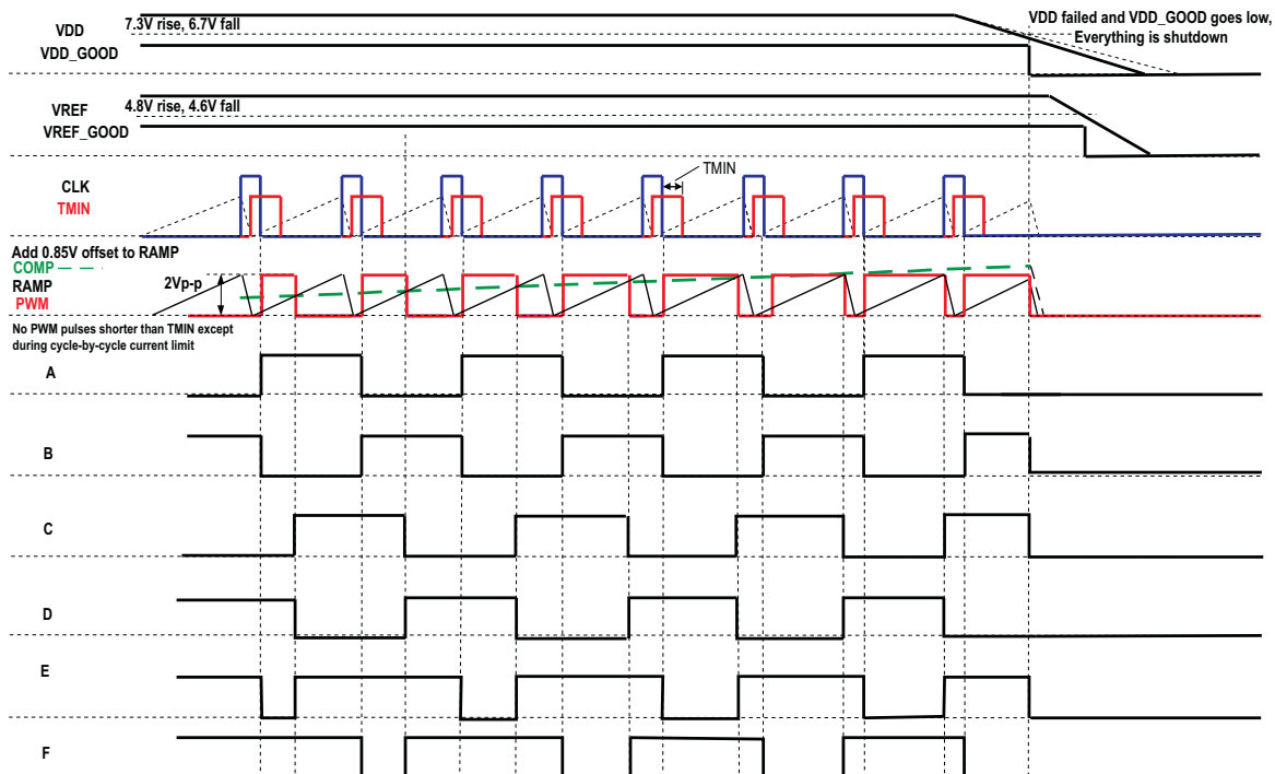
Figure 2. UCC28951-Q1 Steady-State and Shutdown Timing Diagram
