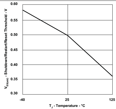
Figure 16. Shutdown, Restart, and Reset Threshold vs Temperature
