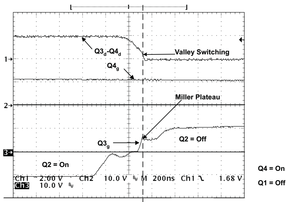
Figure 16. V_{IN} = 390 V, I_{OUT} = 5 A
