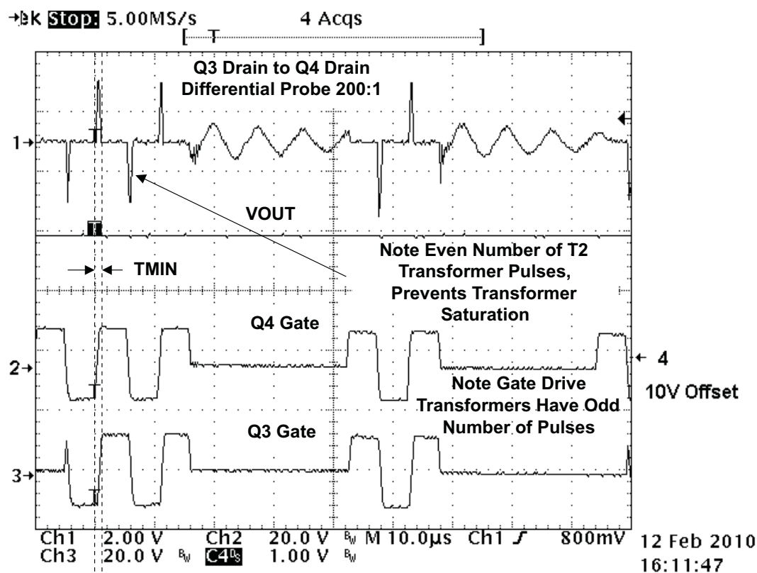
Figure 23. Burst Mode
