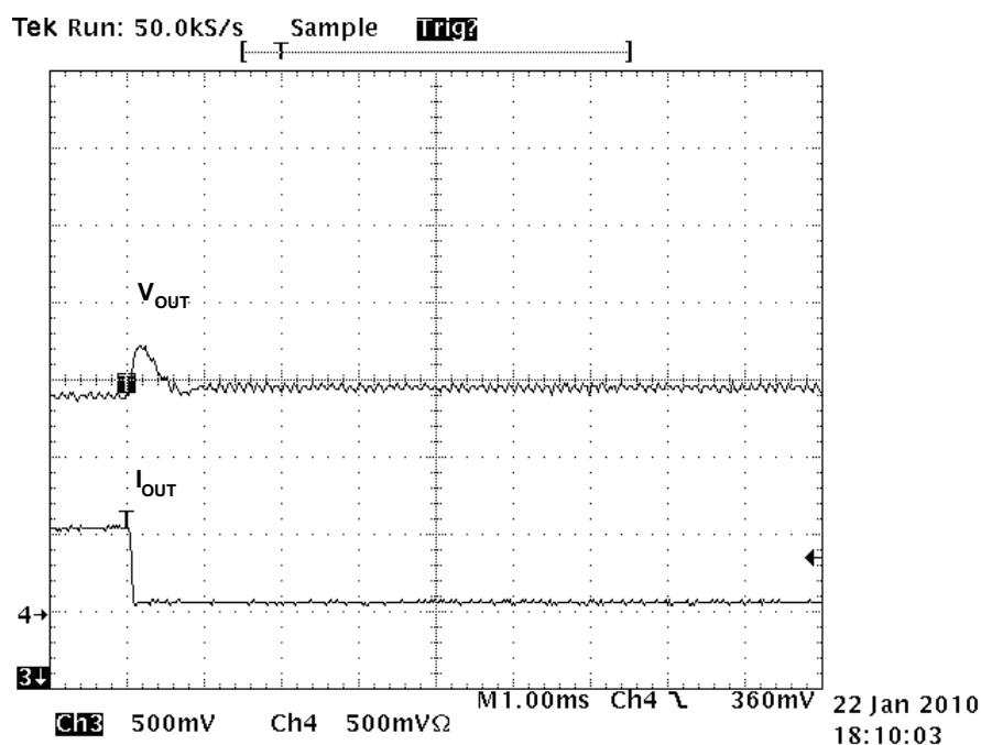
Figure 12. V_{IN} = 390\text{ V} , I_{OUT} = 5\text{ A to } 50\text{ A}
