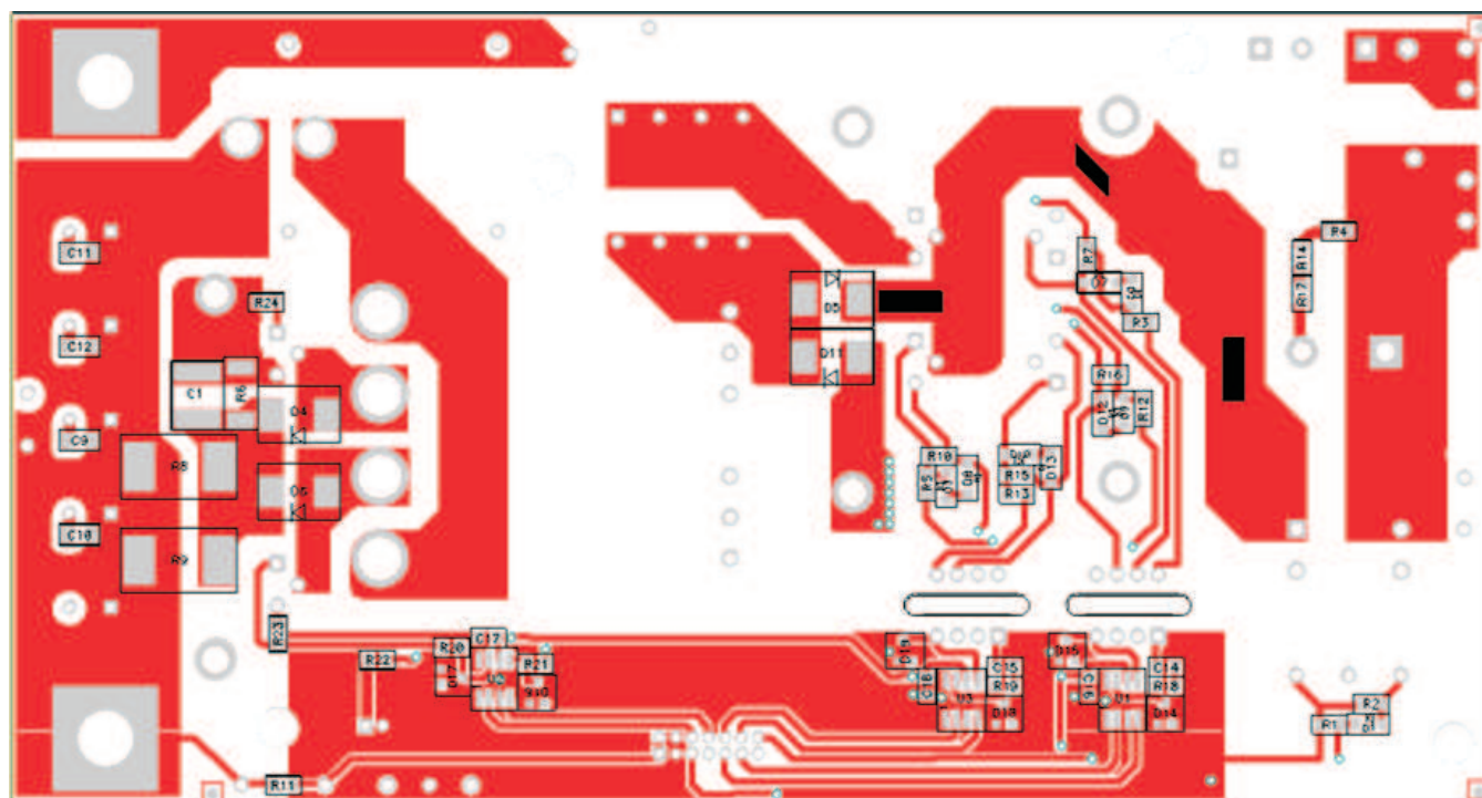
Figure 26. UCC28950EVM-442 Power Stage Bottom Layer Assembly Drawing (bottom view)
