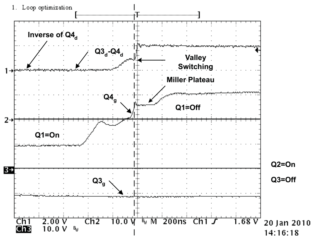
Figure 15. V_{IN} = 390 V, I_{OUT} = 5 A
