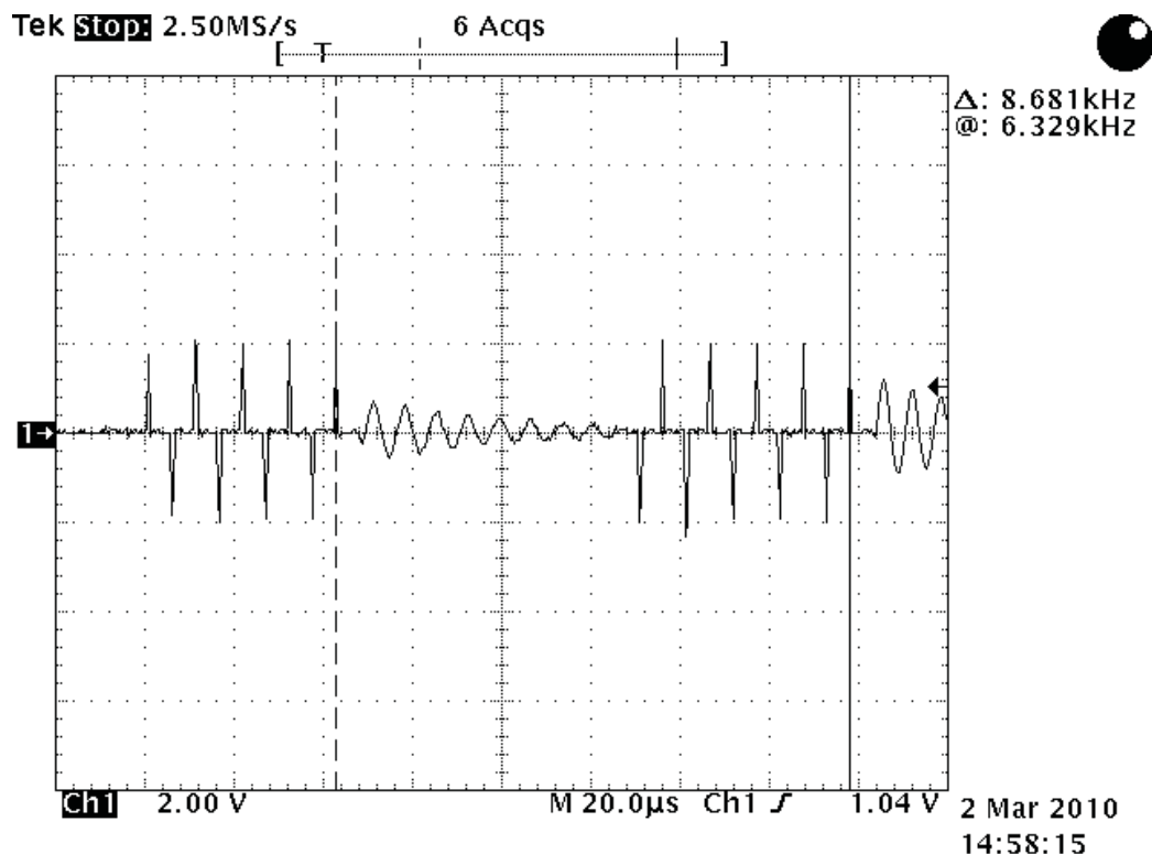
Figure 24. Burst Mode
