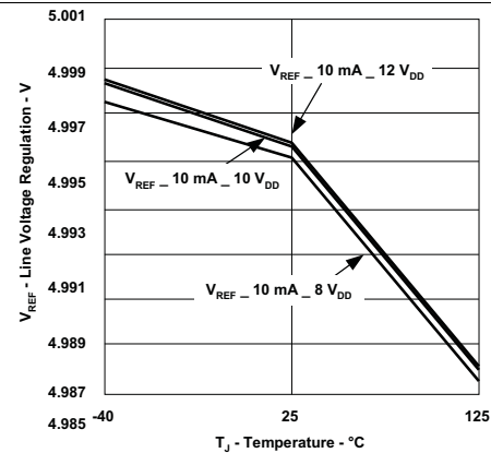
Figure 8. Line Voltage Regulation (I_LOAD = 10 mA) vs Temperature
