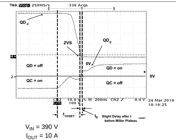
Figure 60. Full-Bridge Gate Drives and Switch Nodes (QD g and QD d )
