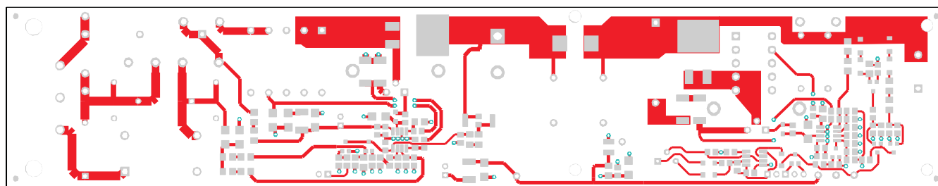
Figure 10. UCC28810EVM-002 Top Copper (top view)
