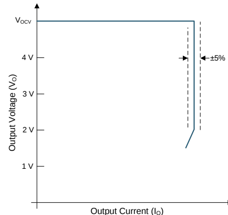
Typical V-I Diagram
