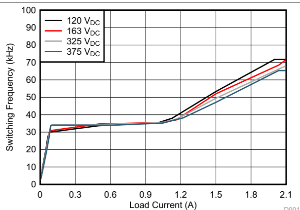
Figure 26. Control Law
