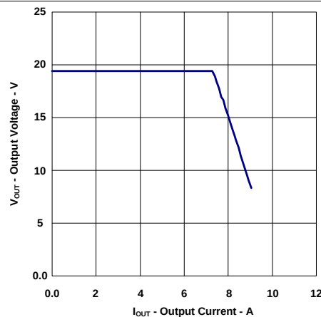
Figure 22. Output Voltage vs. Output Current
