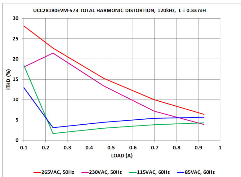
Figure 5. UCC28180EVM-573 Total harmonic Distortion (as a function of line voltage and load current)
