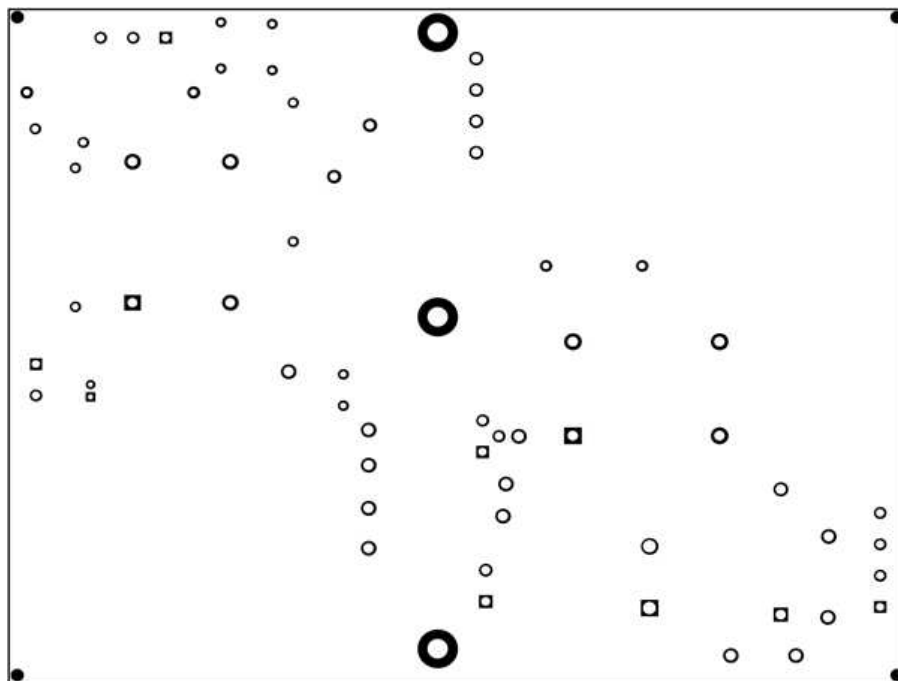
Figure 24. UCC28180EVM-573 Top Copper (top view)
