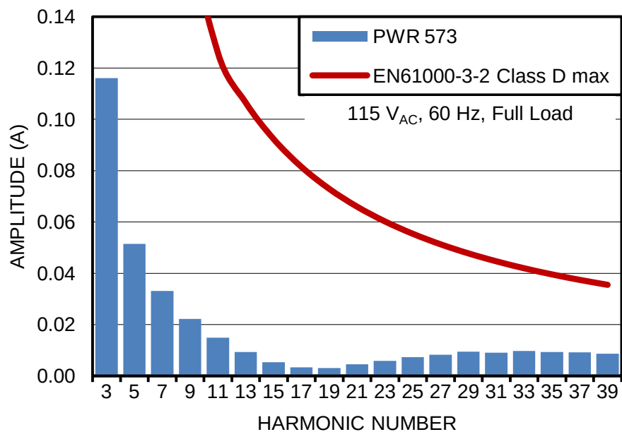
Figure 10. UCC28180EVM-573 Current Harmonics, (115-V AC , 60-Hz input, full load, without the fundamental)
