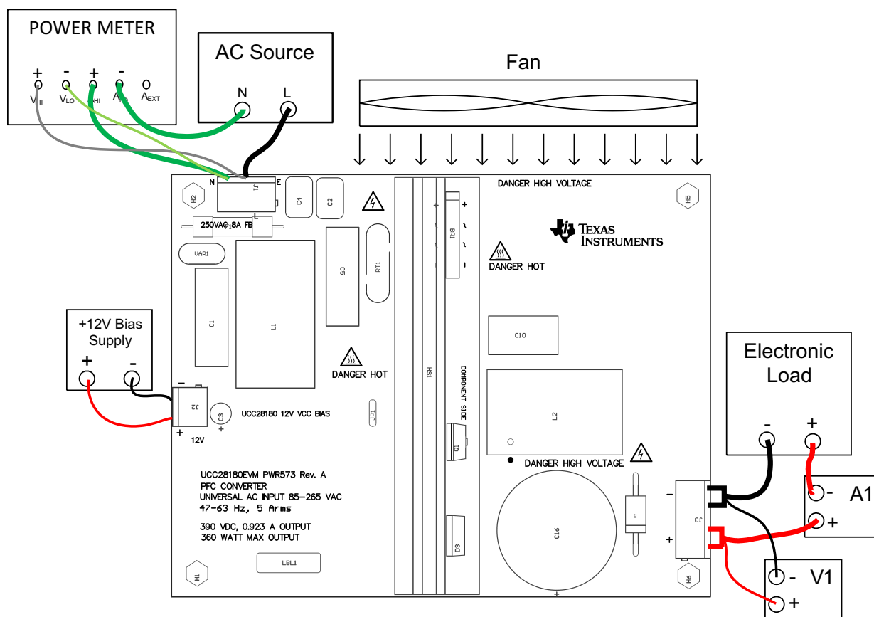
Figure 2. UCC28180EVM-573 Recommended Test Set Up
