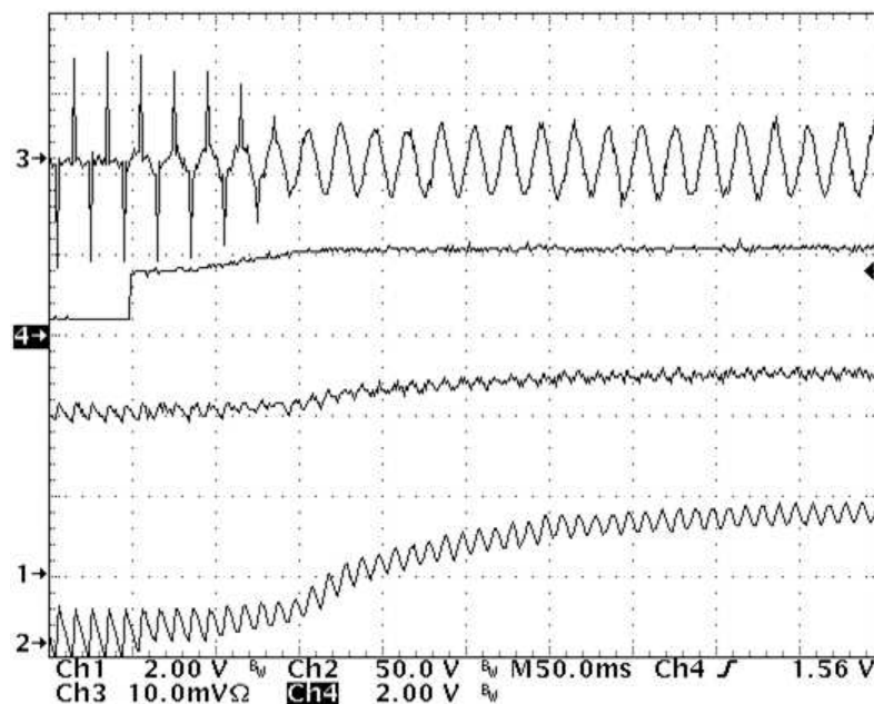
Figure 18. UCC28180EVM-573 Start-Up Waveform (230-V AC , 50-Hz input, full load, CH 1 = V SENSE at 2 V/div, CH 2 = V OUT at 50 V/div., offset by 300 V, CH 3 = I IN at 5 A/div., CH 4 = V COMP at 2 V/div.)
