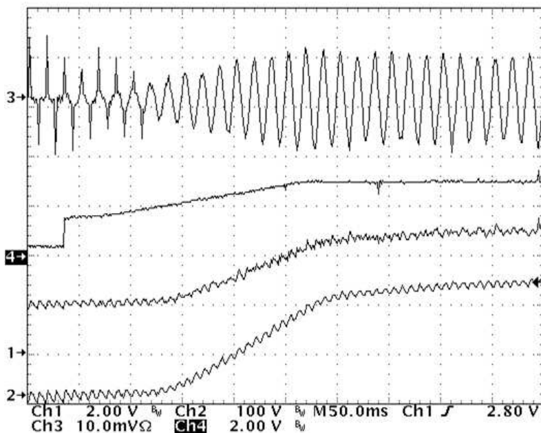
Figure 17. UCC28180EVM-573 Start-Up Waveform (115-V AC , 60-Hz input, full load, CH 1 = V SENSE at 2 V/div, CH 2 = V OUT at 100 V/div., offset by 150 V, CH 3 = I IN at 5 A/div., CH 4 = V COMP at 2 V/div.)
