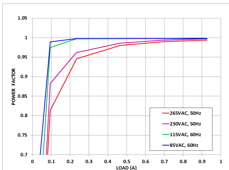
Figure 4. UCC28180EVM-573 Power Factor (as a function of line voltage and load current)
