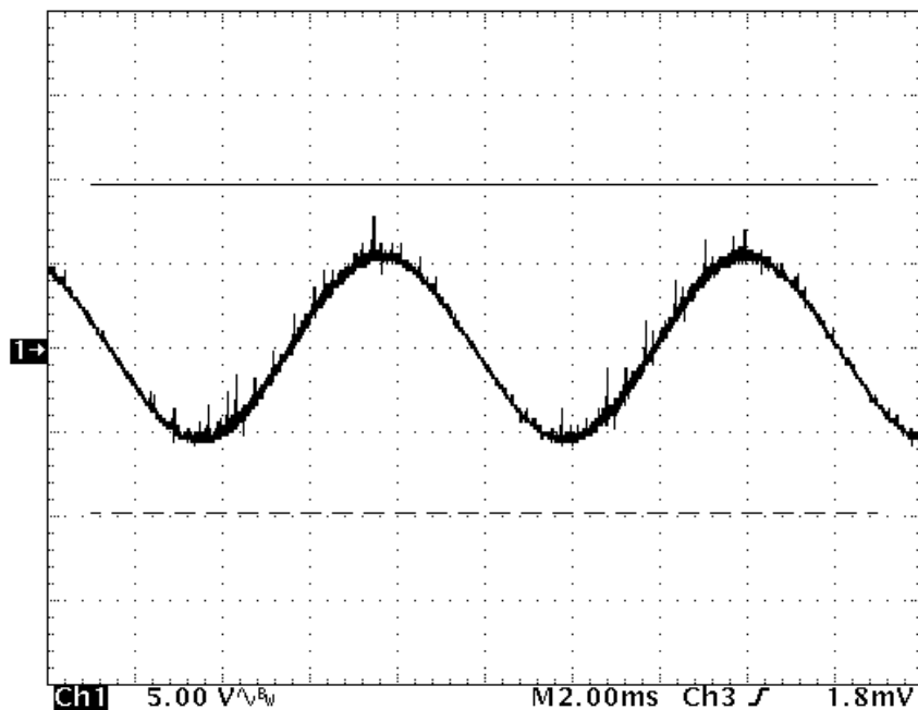
Figure 13. UCC28180EVM-573 Line Frequency Output Voltage Ripple (115 V AC , 60 Hz input, full load)
