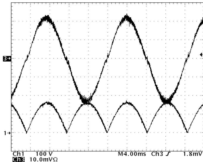
Figure 12. UCC28180EVM-573 Input Current and Input Voltage at the Output of the Bridge Rectifier, (230 V_{AC} , 50 Hz, full load. (CH 1 = rectified input voltage on BR1, 100 V/div., CH 3 = I_{IN} 1 A/div.))
