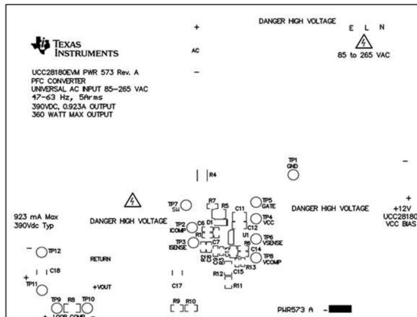
Figure 23. UCC28180EVM-573 Bottom Layer Assembly Drawing (bottom view)
