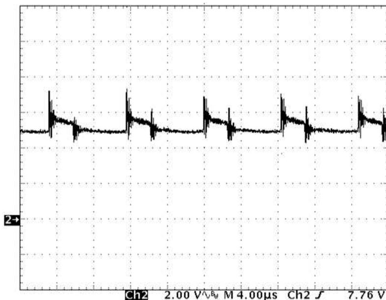
Figure 15. UCC28180EVM-573 Switching Frequency Output Voltage Ripple (115 V AC , 60 Hz input, full load)
