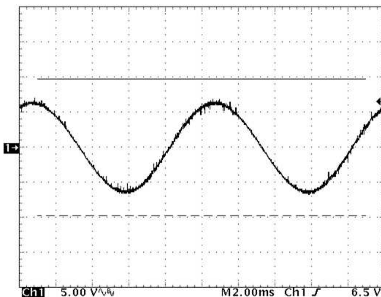
Figure 14. UCC28180EVM-573 Line Frequency Output Voltage Ripple (230 V AC , 50 Hz input, full load)
