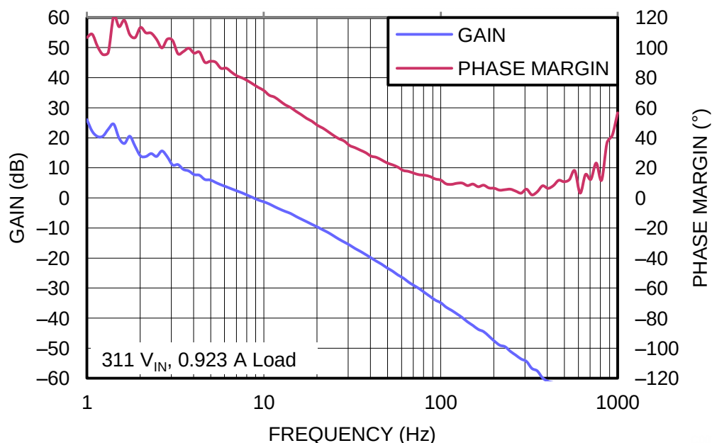
Figure 21. UCC28180EVM-573 Voltage Loop Response Gain and Phase, (162-V DC , full load, f_{co} = 8.6 -Hz, phase margin = 63 degrees)
