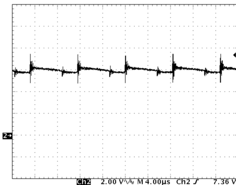
Figure 16. UCC28180EVM-573 Switching Frequency Output Voltage Ripple (230 V AC , 50 Hz input, full load)
