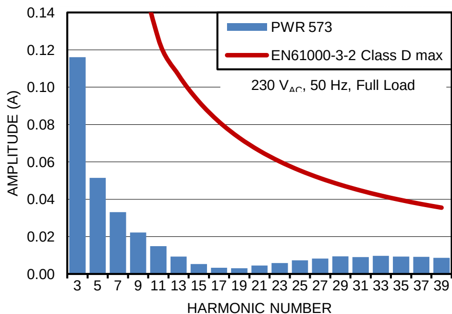
Figure 9. UCC28180EVM-573 Current Harmonics, (230-V AC , 50-Hz input, full load, without the fundamental)
