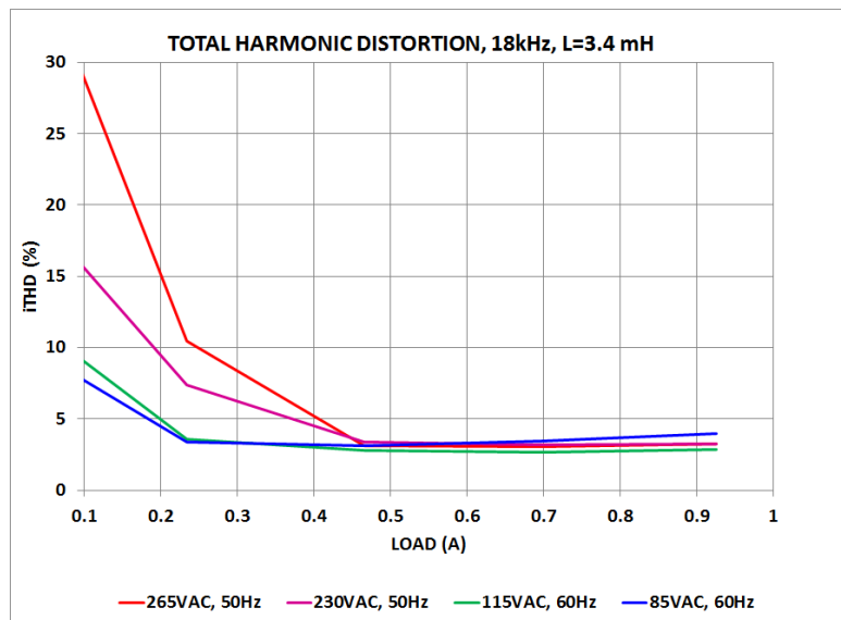
Figure 7. Total harmonic distortion (as a function of line voltage and load current) with L = 3.4 mH and f_{SW} = 18 kHz
