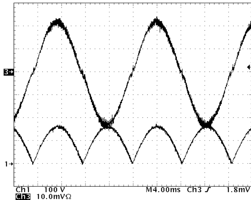
Figure 11. UCC28180EVM-573 Input Current and Input Voltage at the Output of the Bridge Rectifier, (115- V_{AC} , 60 Hz, full load. (CH 1 = rectified input voltage on BR1, 100 V/div., CH 3 = I_{IN} 2 A/div.))
