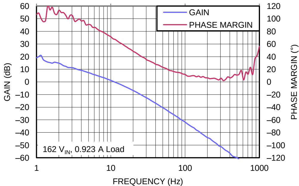
Figure 20. UCC28180EVM-573 Voltage Loop Response Gain and Phase, (311-V DC , full load, f_{co} = 10.7 -Hz, phase margin = 68 degrees)
