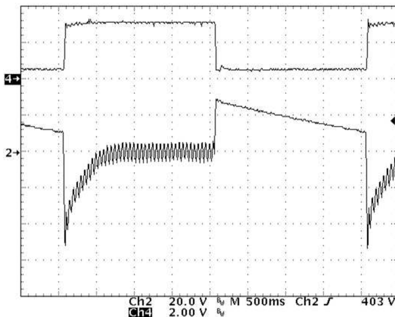
Figure 19. Load Transient
