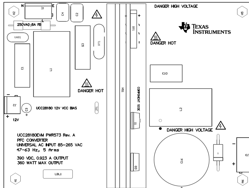
Figure 22. UCC28180EVM-573 Top Layer Assembly Drawing (top view)
