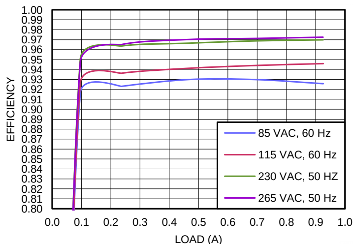
Figure 3. UCC28180EVM-573 Efficiency (as a function of line voltage and load current)
