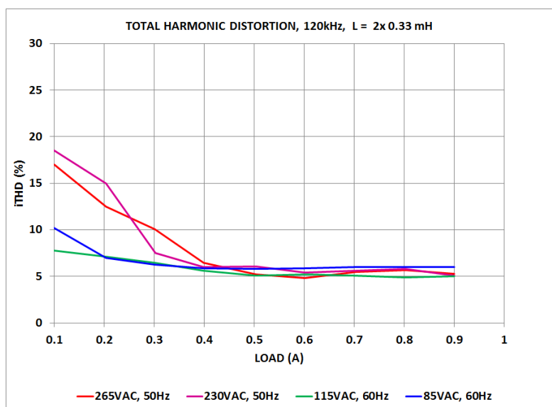
Figure 6. Total Harmonic Distortion with 2x Inductance
