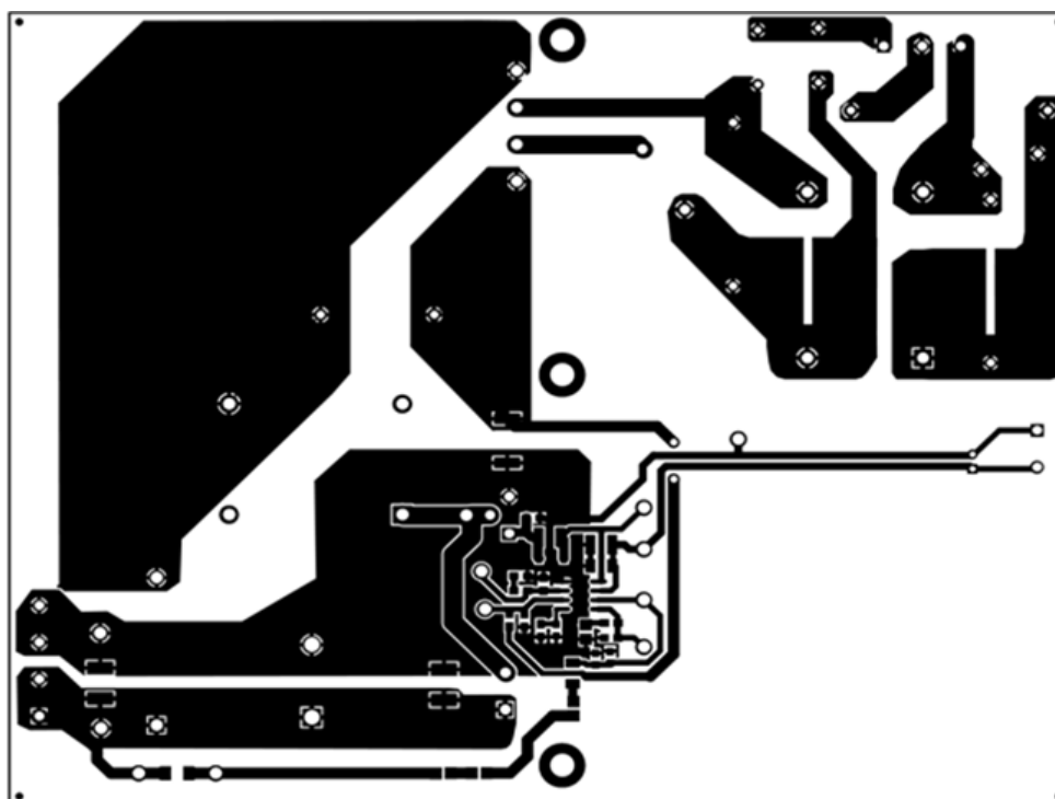
Figure 25. UCC28180EVM-573 Bottom Copper (bottom view)
