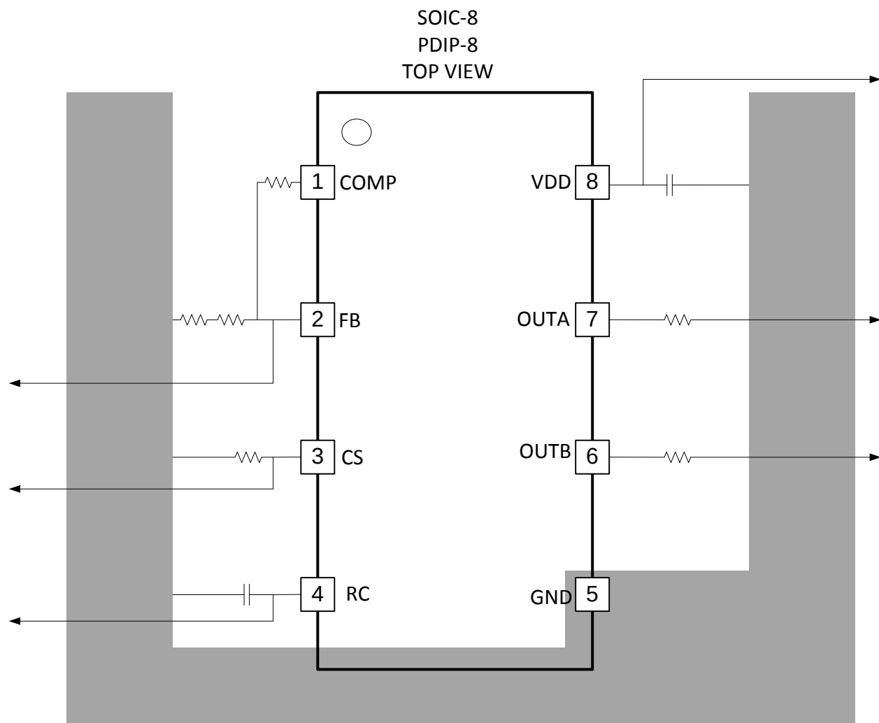
Figure 9. Layout Example
