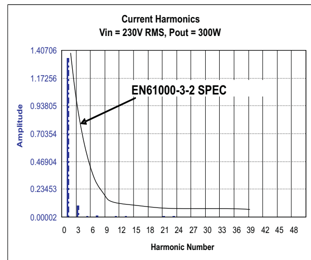
Figure 7. Current Harmonics
