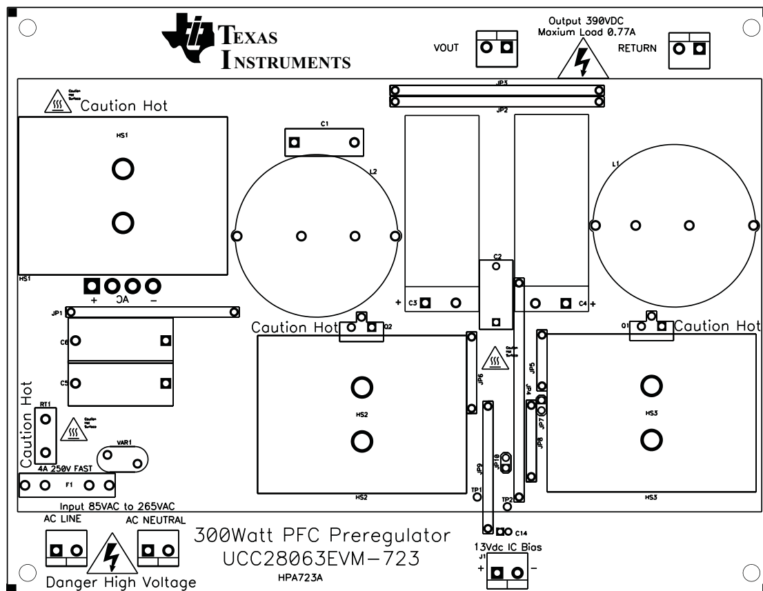
Figure 20. Top Layer Assembly
