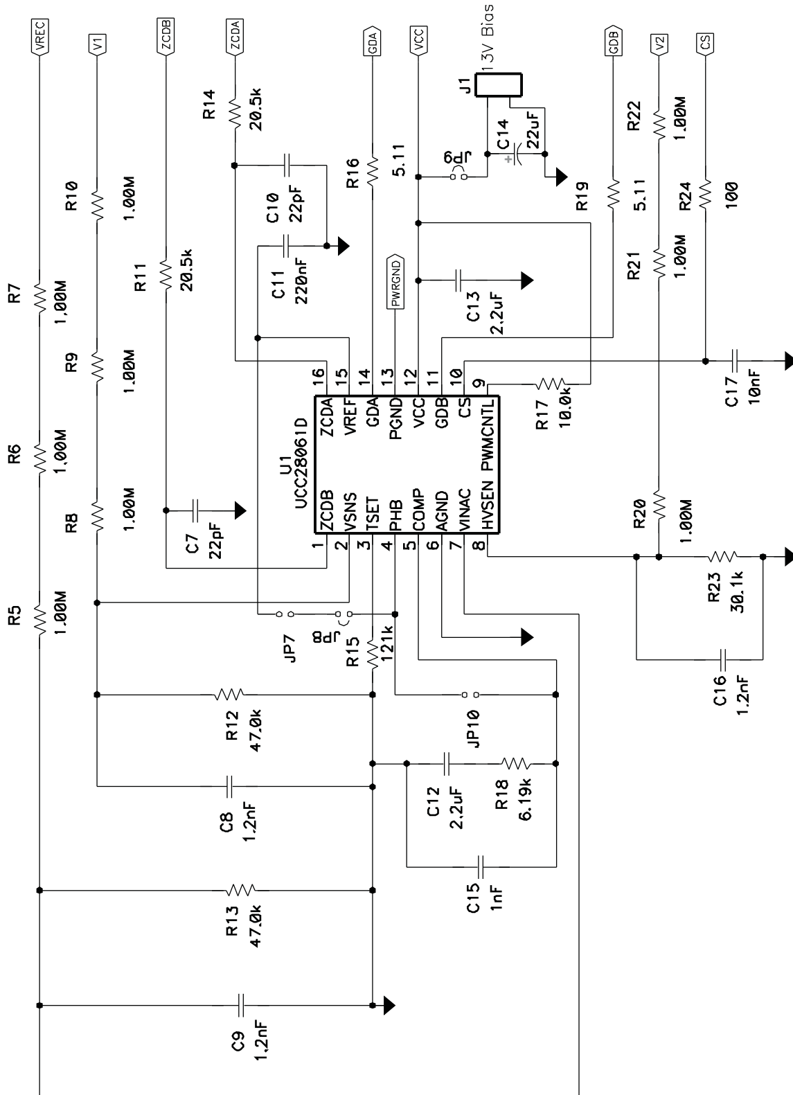
Figure 2. Controller Circuitry
