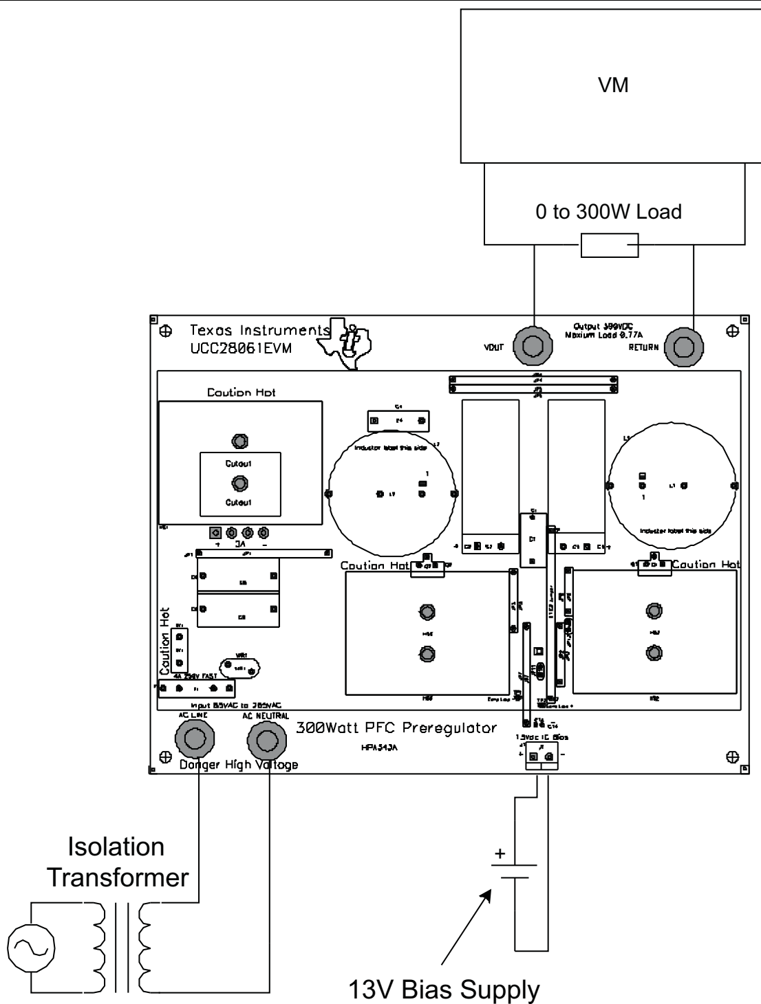
Figure 3. Test Setup
