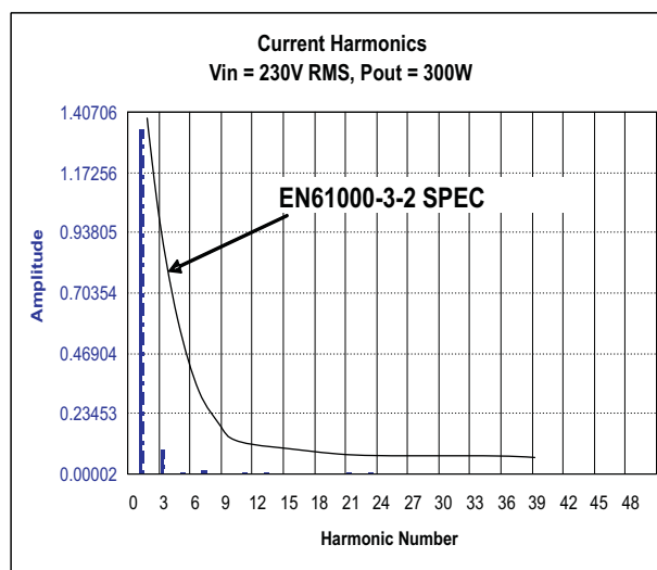
Figure 7. Current Harmonics
