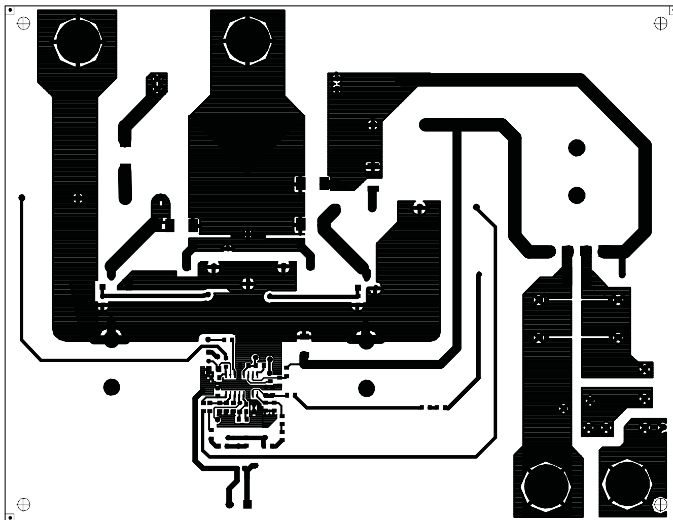
Figure 21. Bottom Layer Copper
