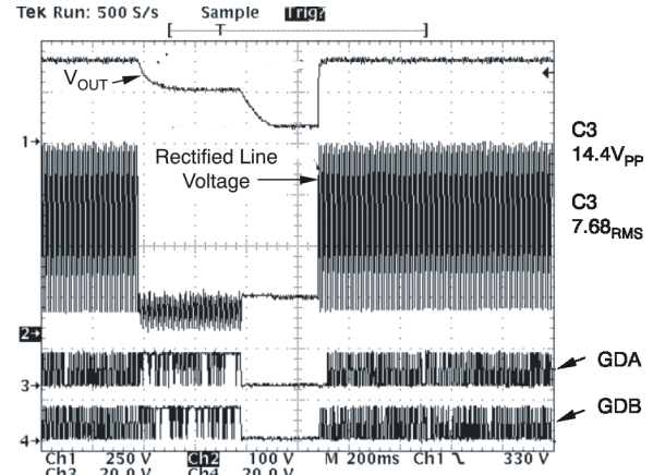
Figure 18. Brownout at 265 V_{RMS}
