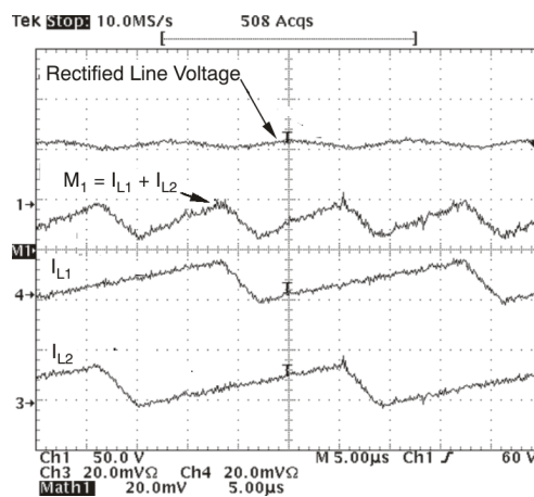
Figure 10. Inductor and Input Ripple Current at 85\text{ V}_{RMS} Input at Half the Line Voltage
