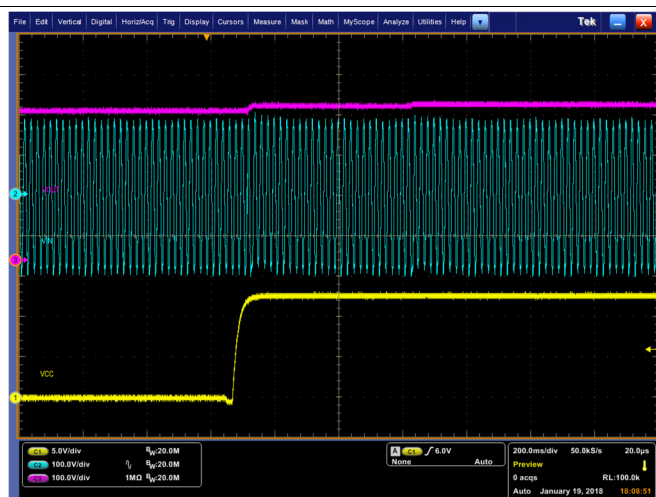
Figure 12. 265 VAC Start-up No Load
