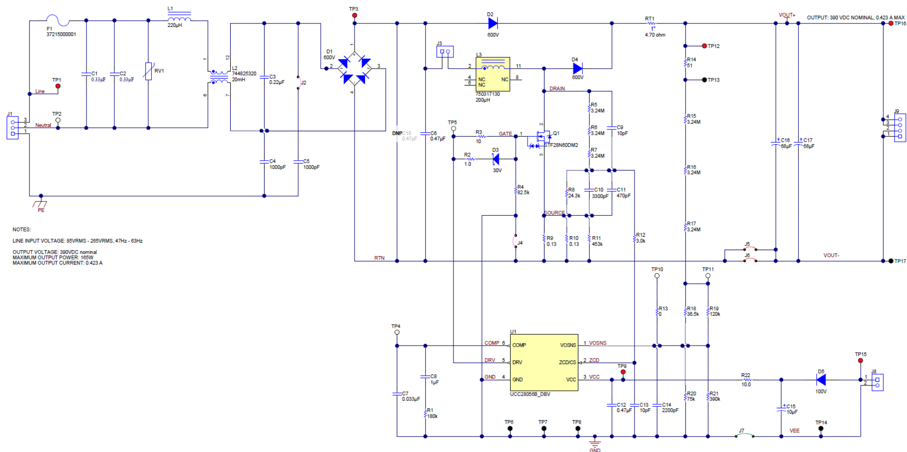
Figure 22. UCC28056BEVM-296 Schematic
