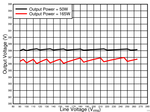
Figure 4. Line Regulation versus Input Voltage
