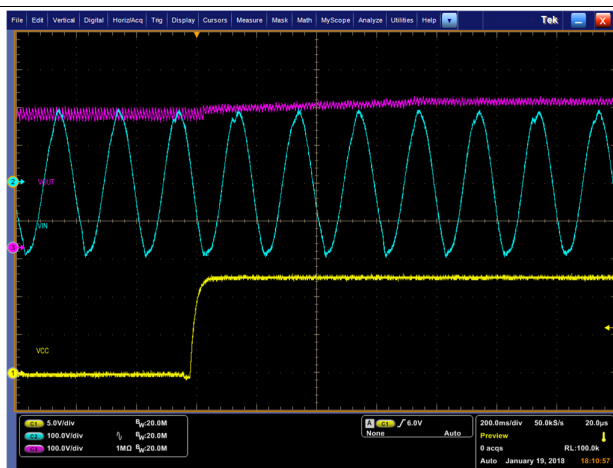
Figure 13. 265 VAC Start-up Full Load
