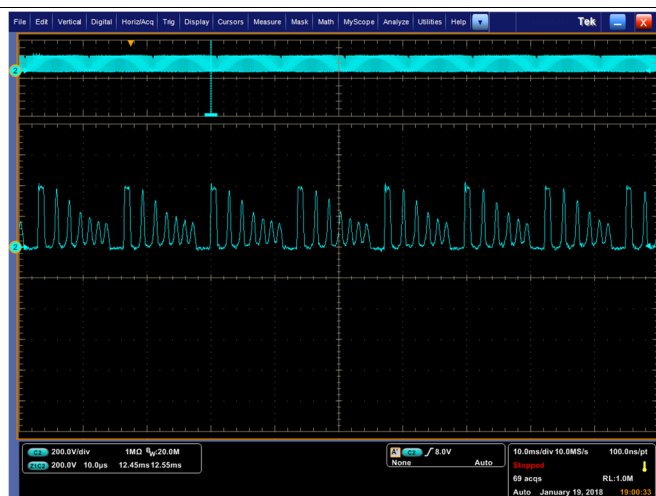
Figure 19. 265 VAC Valley Switching 100-mA Load
