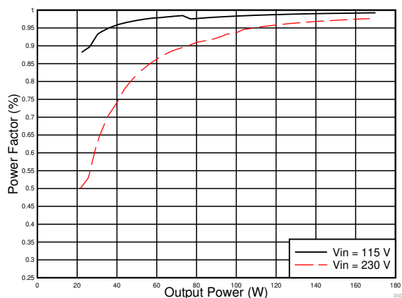
Figure 5. Power Factor versus Output Power
