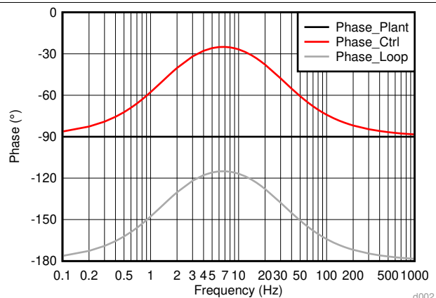
Figure 32. Phase vs Frequency
