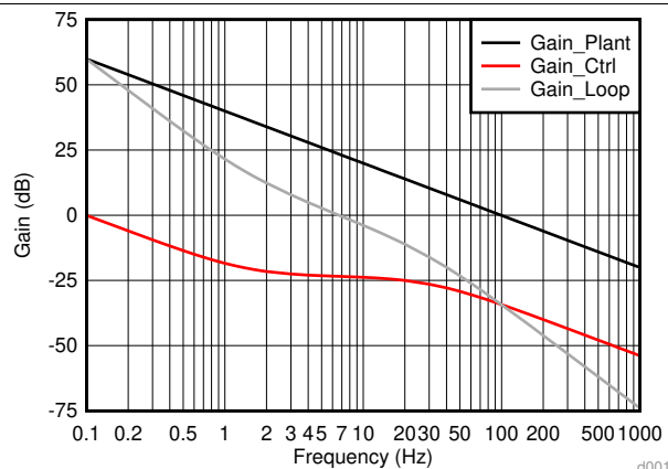
Figure 31. Gain vs Frequency
