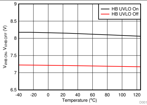
Figure 14. VHB-VHS UVLO Thresholds vs Temperature
