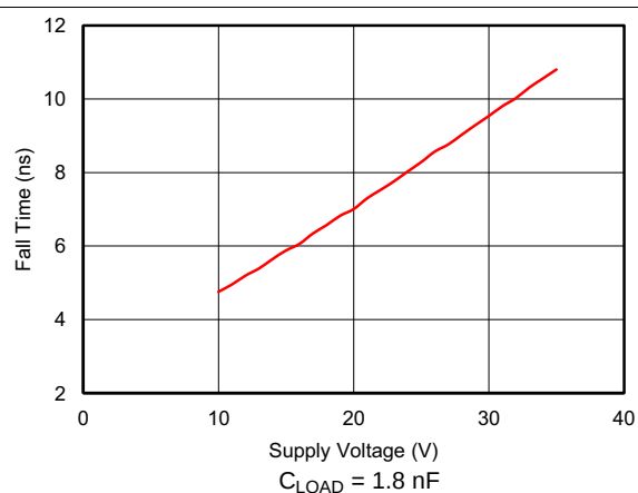
Figure 5. Fall Time vs. Supply Voltage
