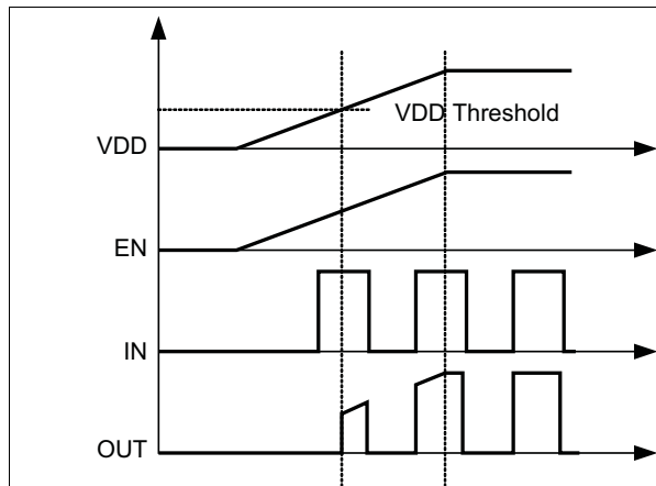
Figure 26. Power up Non-Inverting Driver
