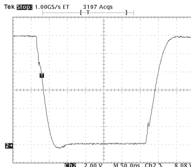
Figure 29. Pulse Response
