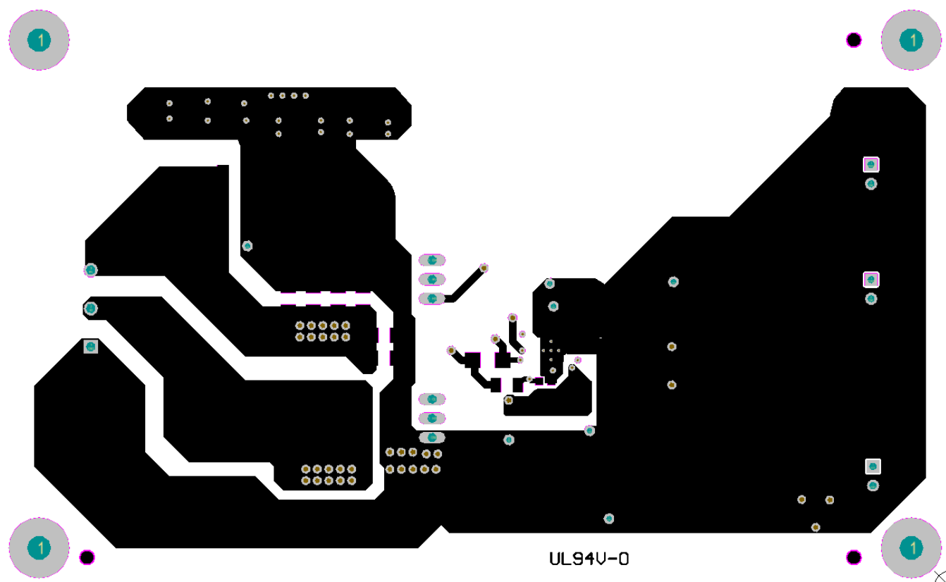
Figure 14. Bottom Layer
