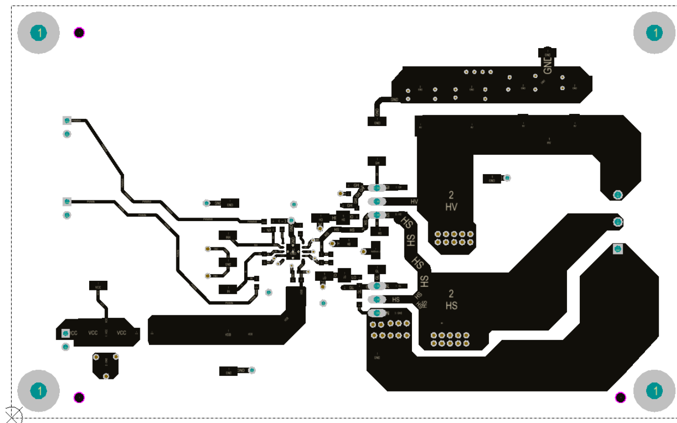
Figure 12. Top Layer
