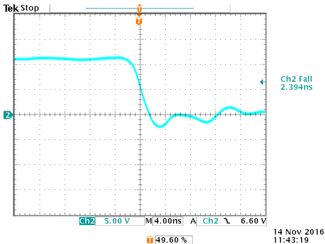
Figure 3. HO Fall Time
