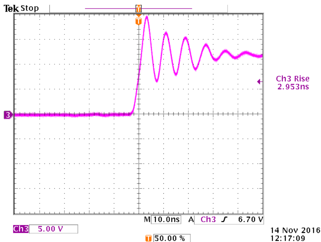
Figure 4. LO Rise Time
