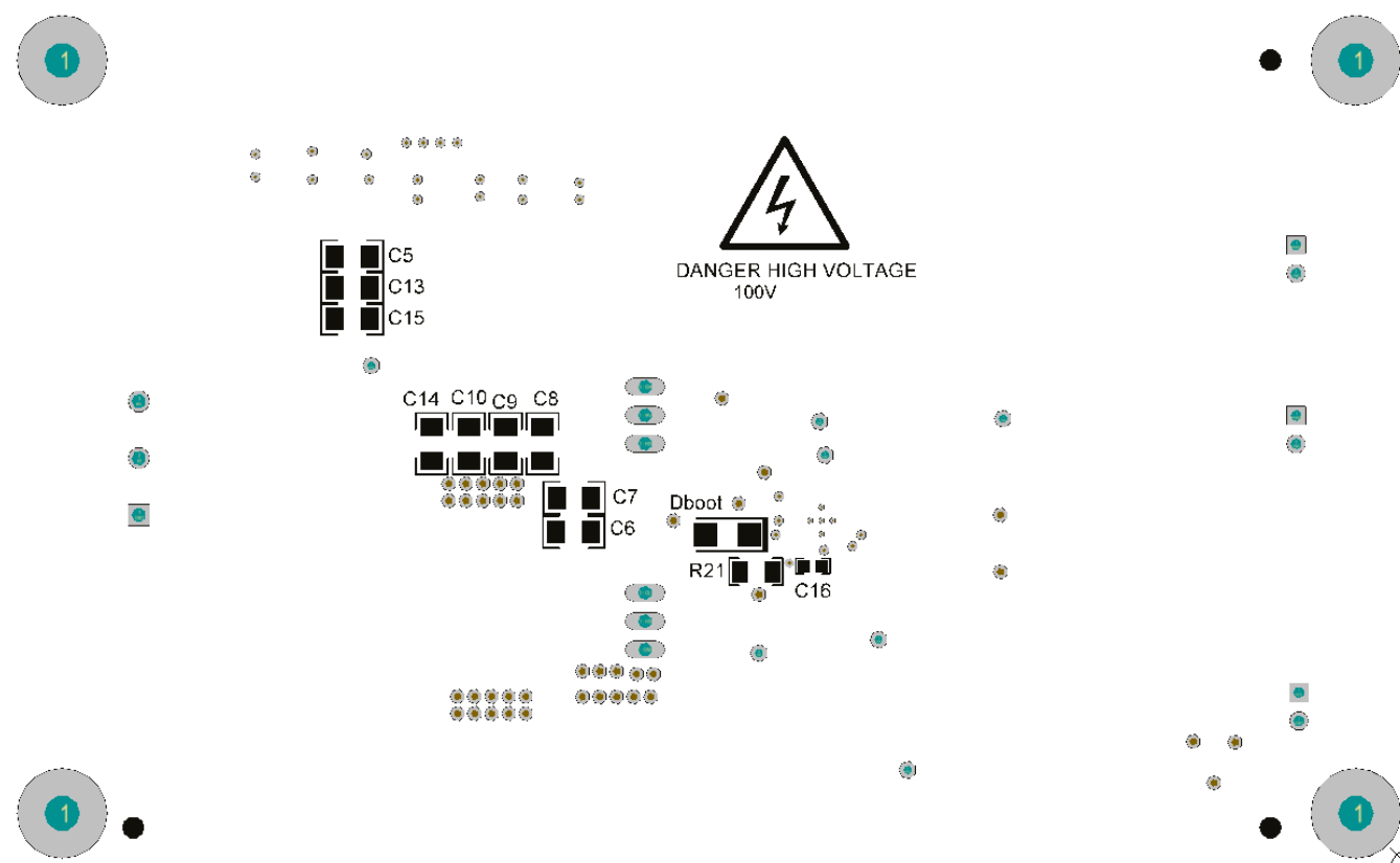
Figure 13. Bottom Overlay
