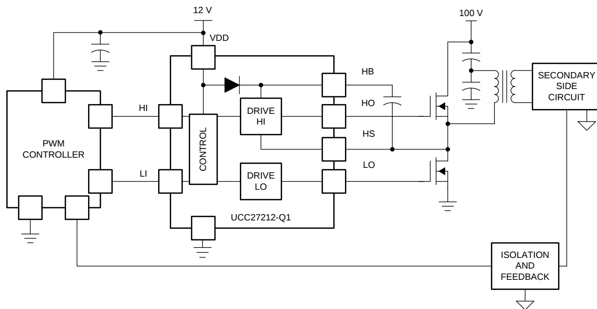
Figure 19. UCC27212 Typical Application
