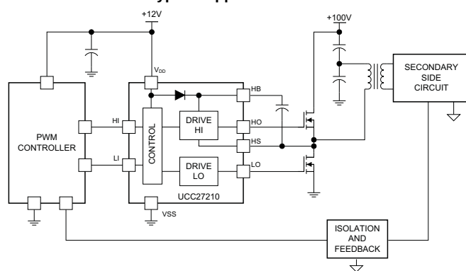
Typical Application: UCC27210
