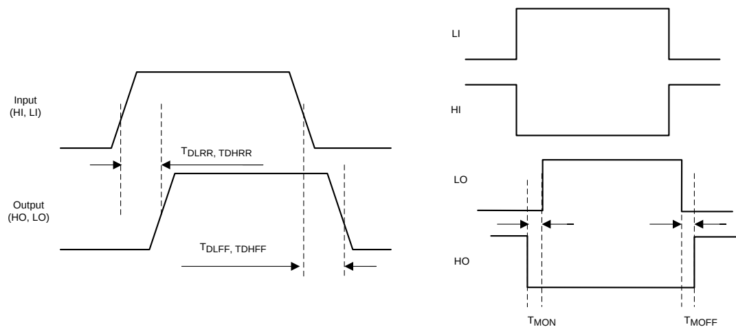
Figure 1. Timing Diagrams
