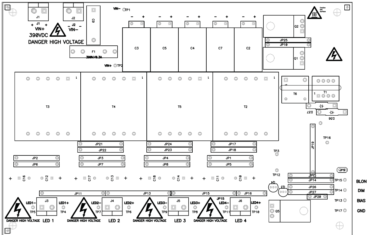
Figure 17. Top Assembly
