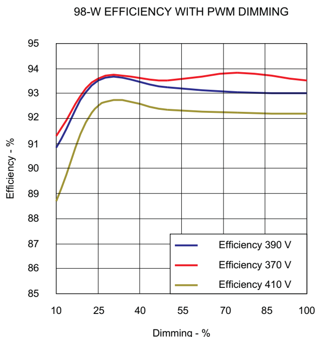
Figure 8. Efficiency 10% to 100% PWM Dimming
