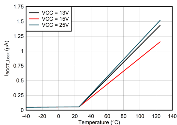
Figure 5. I_{BOOT\_LEAK} vs Temperature
