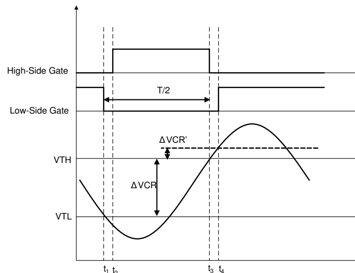
Figure 27. HHC Gate On/Off Control Principle
