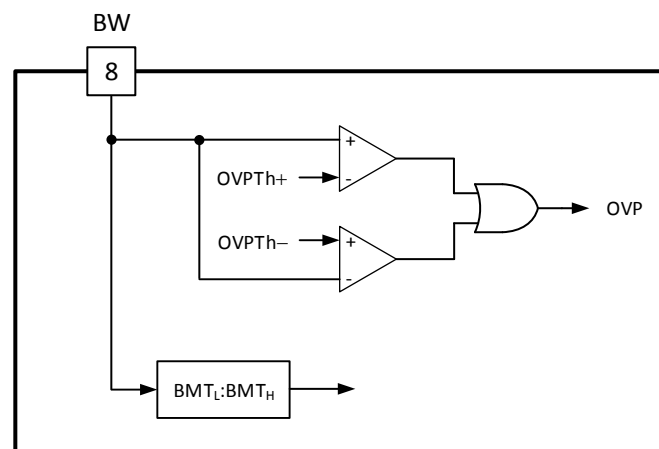
Figure 34. Bias Winding Sensing Block Diagram
