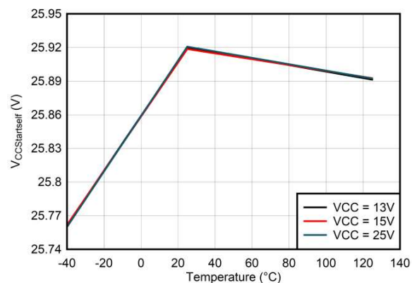
Figure 24. V_{CCStartself} vs Temperature
