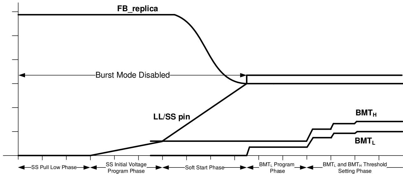
Figure 45. Timing Diagram of LL/SS Pin Programming
