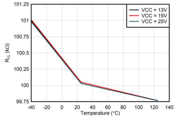
Figure 8. R_{\text{LL}} vs Temperature
