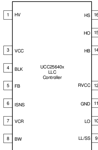
DDB Package 16-Pin SOIC (Pins 2, 13 removed) Top View
