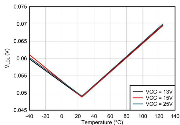
Figure 20. V_{LOL} vs Temperature
