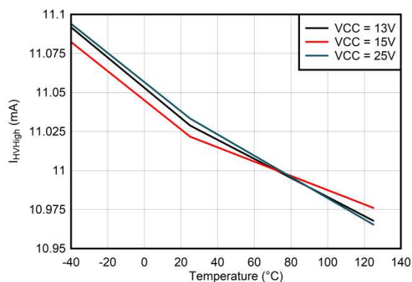
Figure 1. I_{HVHigh} vs Temperature
