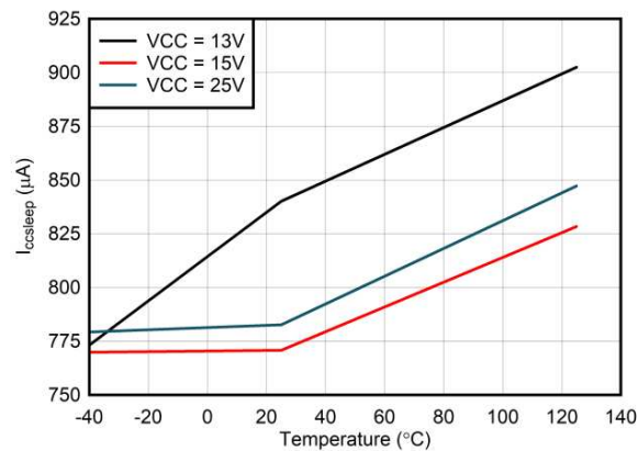
Figure 11. I_{\text{CCSleep}} vs Temperature
