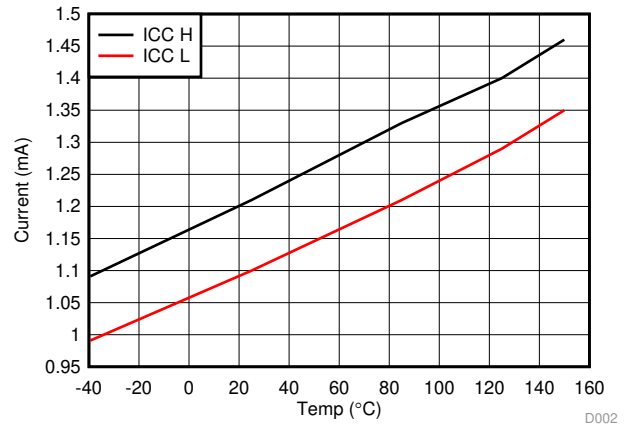
Figure 5. Supply currents versus Temperature
