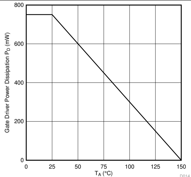
Figure 2. Thermal Derating Curve for Limiting Power per VDE
