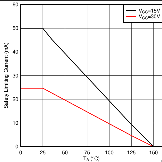
Figure 1. Thermal Derating Curve for Limiting Current per VDE
