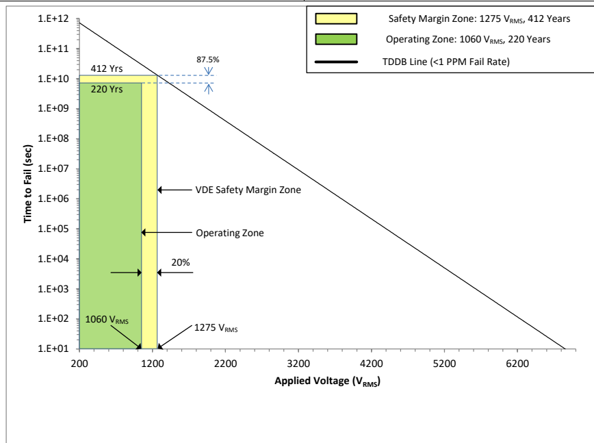
Figure 3. Reinforced Isolation Capacitor Life Time Projection
