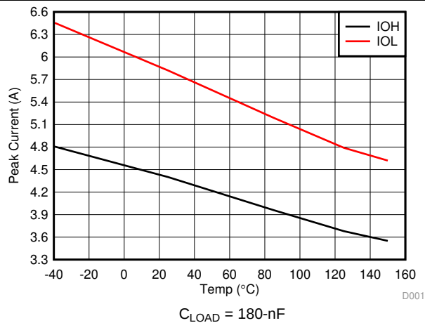
Figure 4. Output Drive currents versus Temperature
