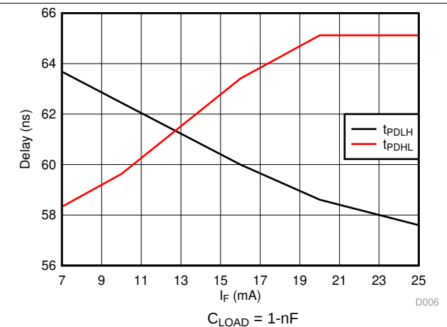
Figure 9. Propagation delay versus Forward current
