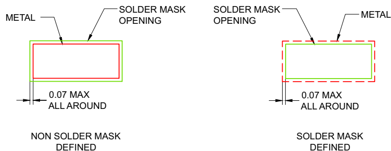
SOLDER MASK DETAILS
