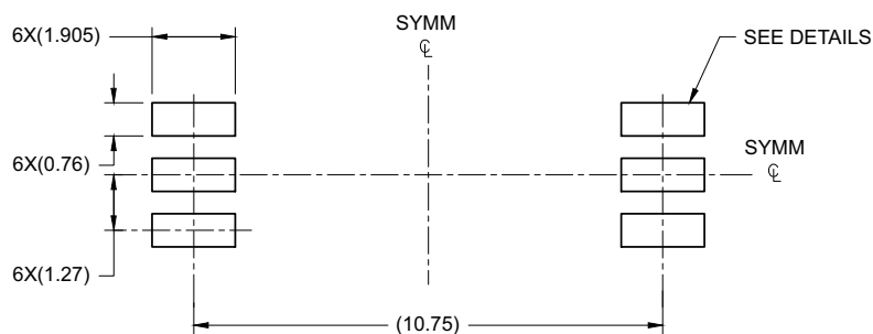
LAND PATTERN EXAMPLE SCALE:6X
