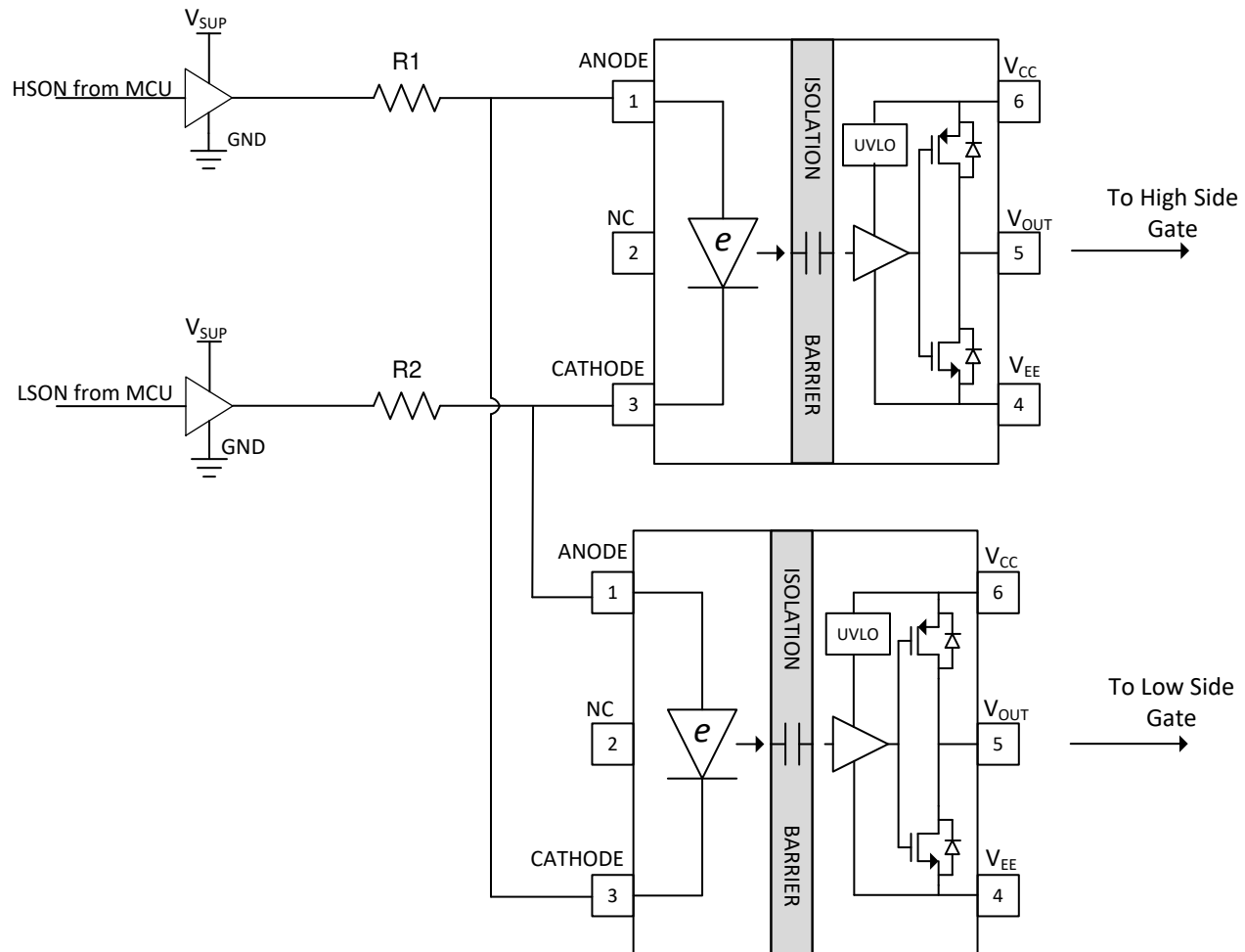
Figure 22. Interlock
