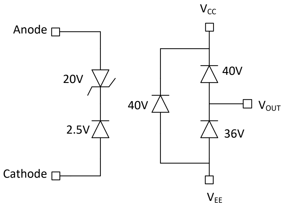
Figure 25. ESD Structure
