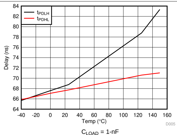
Figure 8. Propagation delay versus Temperature
