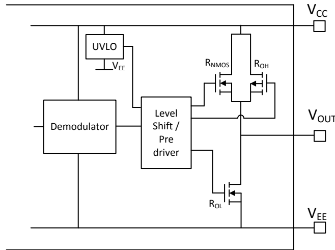
Figure 23. Output Stage
