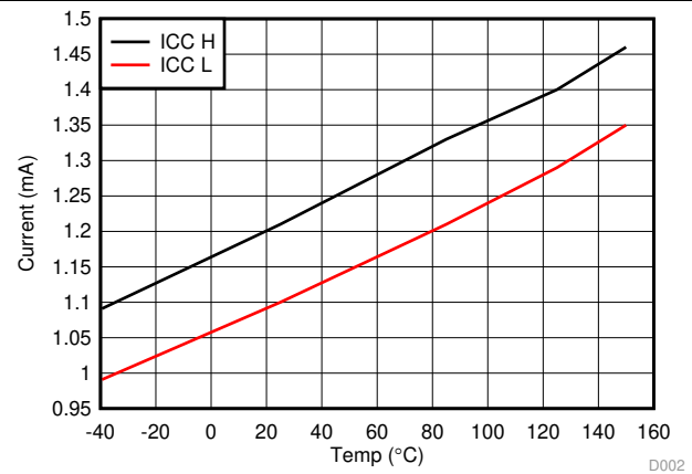
Figure 5. Supply currents versus Temperature
