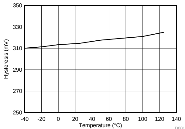
Figure 17. UCC21521ADW UVLO Hysteresis vs. Temperature
