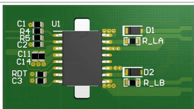
Figure 51. 3-D PCB Bottom View
