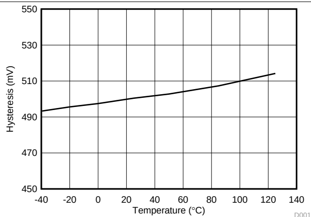
Figure 19. UCC21521DW UVLO Hysteresis vs. Temperature
