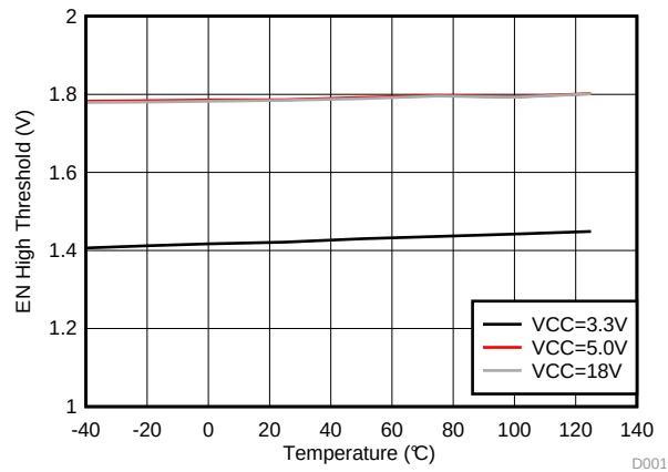
Figure 28. EN High Threshold
