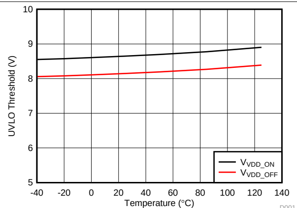
Figure 18. UCC21521ADW UVLO Threshold vs. Temperature
