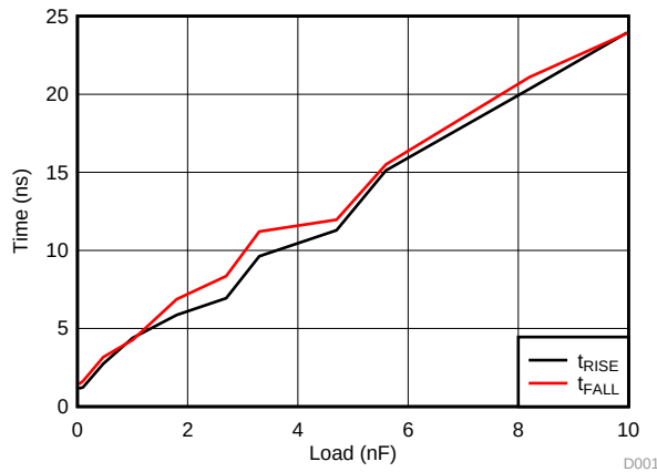
Figure 10. UCC21521ADW and UCC21521DW Rising and Falling Times vs. Load (VDD = 12 V)
