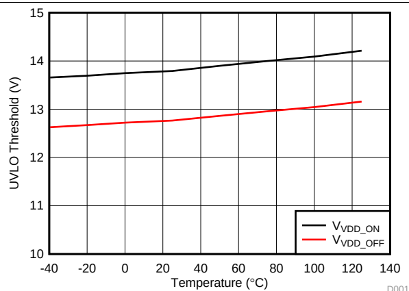
Figure 22. UCC21521CDW UVLO Threshold vs. Temperature
