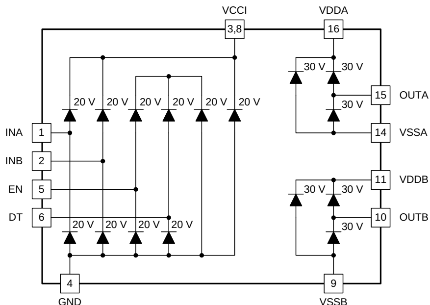
Figure 39. ESD Structure
