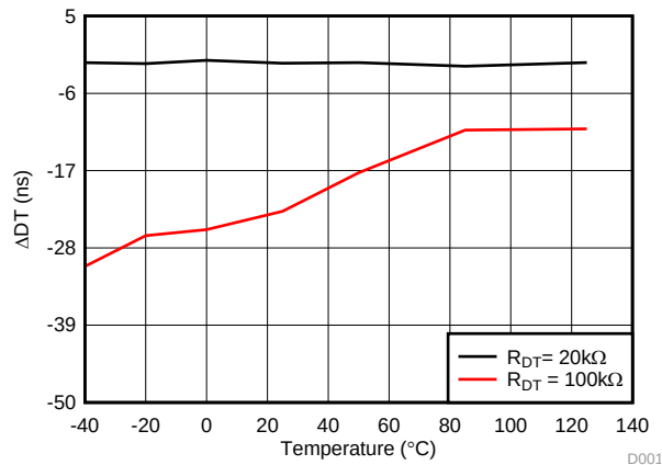
Figure 30. Dead Time Matching vs. Temperature (with R DT = 20 kΩ and 100 kΩ)
