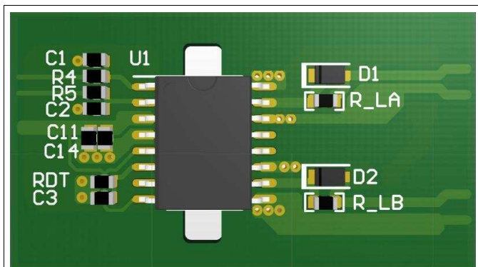
Figure 50. 3-D PCB Top View
