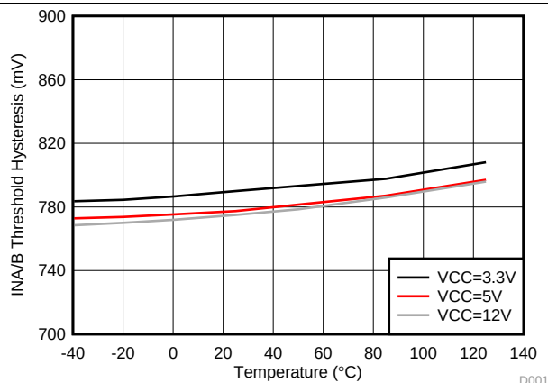
Figure 23. INA/B Hysteresis vs. Temperature
