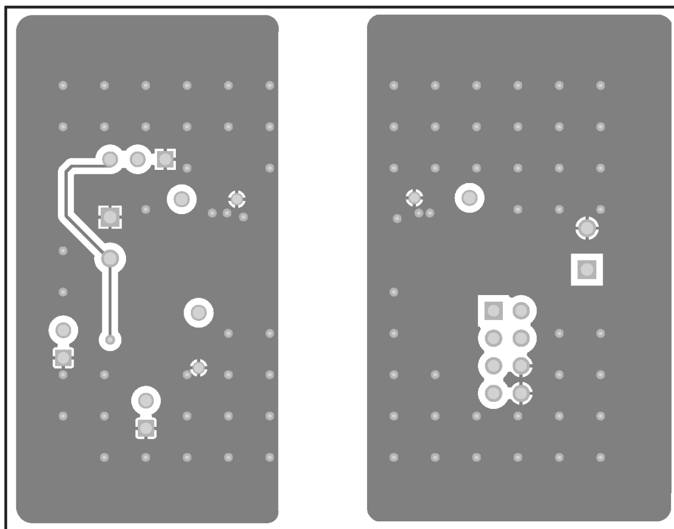
Figure 9. Bottom Layer
