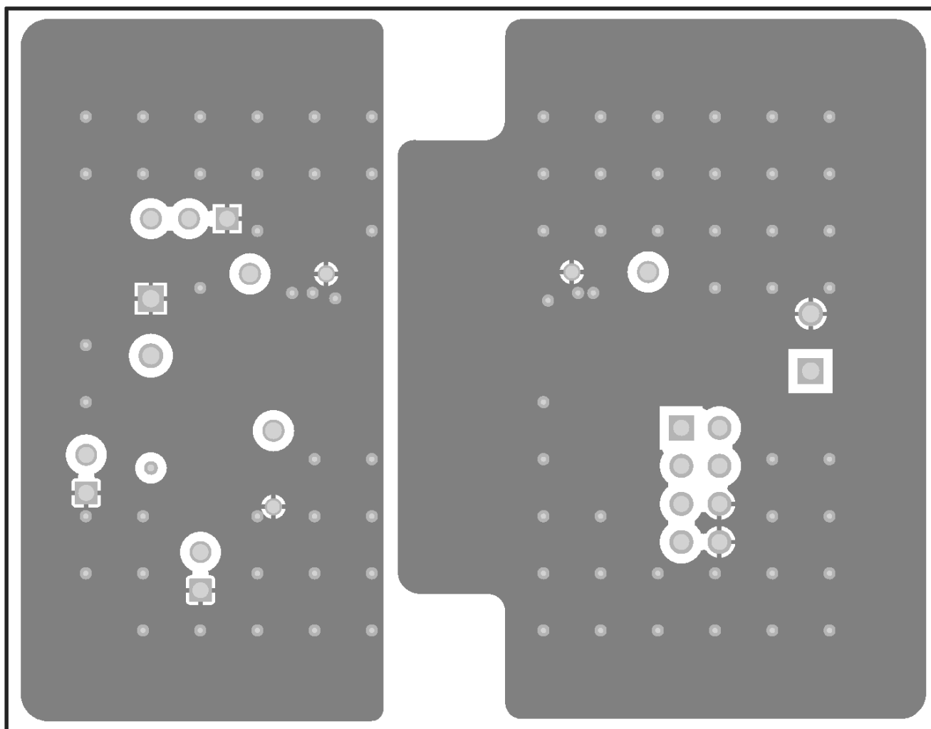
Figure 8. Signal Layer 2
