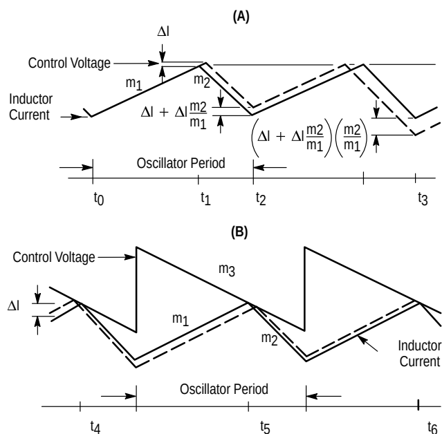
Figure 19. Continuous Current Waveforms
