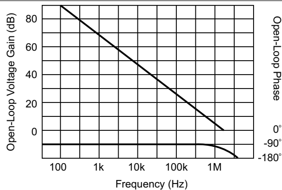
Figure 1. Error Amplifier Gain and Phase vs Frequency
