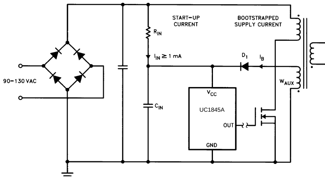
Figure 7. Providing Power to the UC1845A
