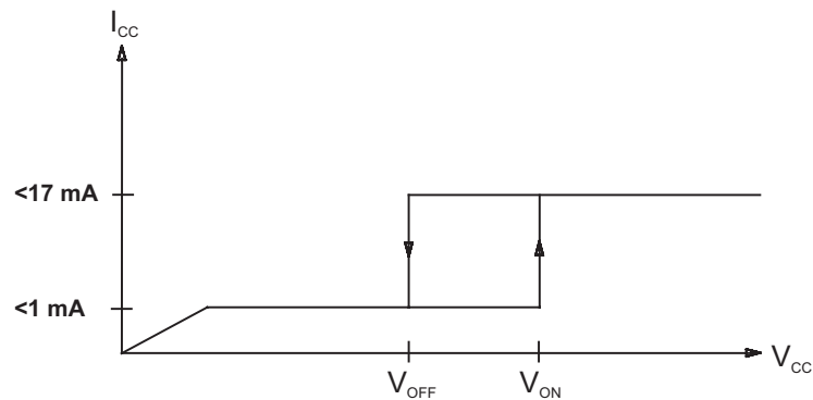
Figure 6. Supply Current Requirements
