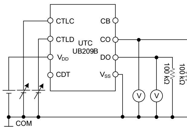
Figure 4. Test Circuit 4
