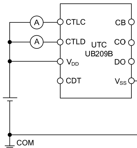
Figure 6. Test Circuit 6
