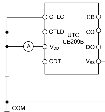
Figure 5. Test Circuit 5
