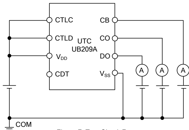
Figure 7. Test Circuit 7
