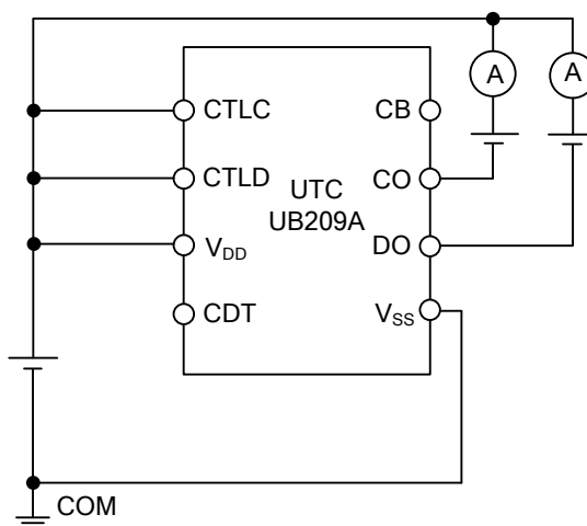
Figure 8. Test Circuit 8
