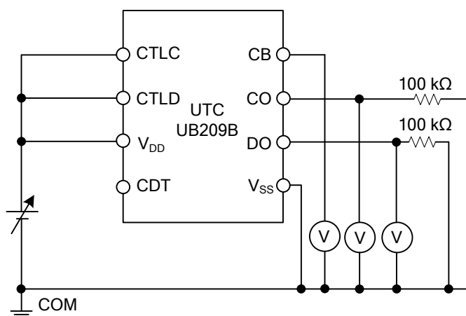
Figure 1. Test Circuit 1
