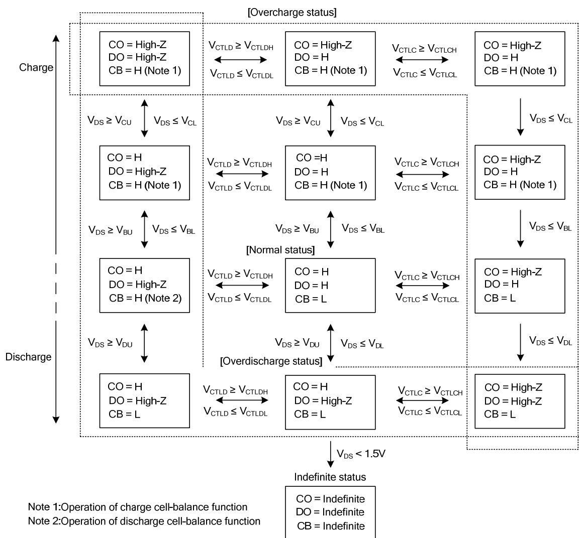
Figure 9. Operation Transition
