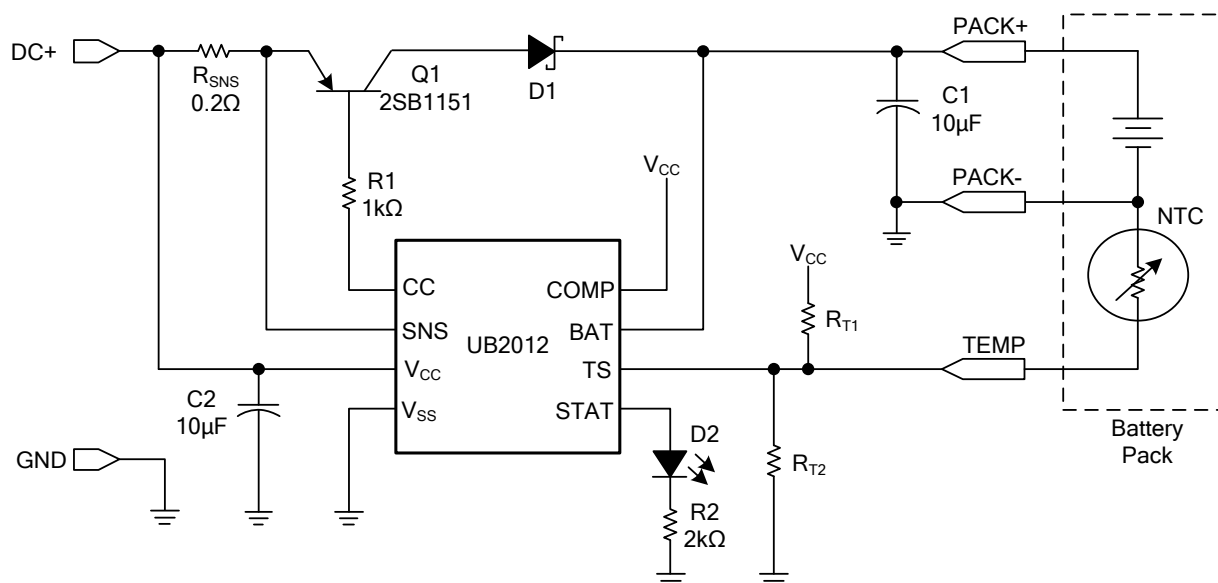
Fig. 1 0.5A Low Dropout Li-Ion/Li-Pol Charger
