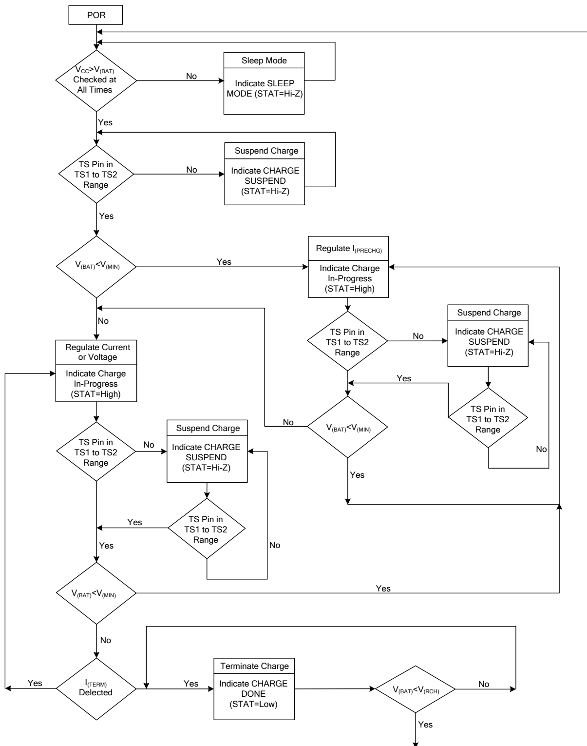
Fig. 2 Operation Flowchart
