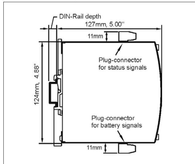
Fig. 21-2 Side view
