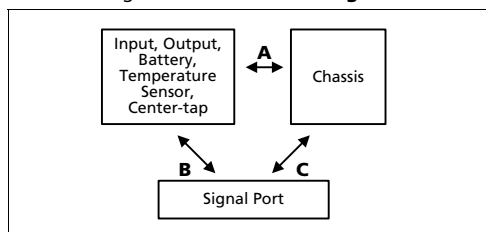
Fig. 19-1 Dielectric strength
