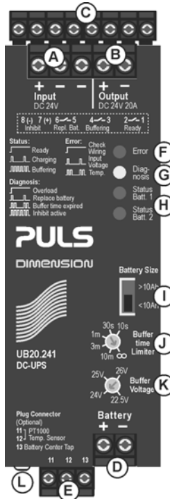
Fig. 14-1 Front side
