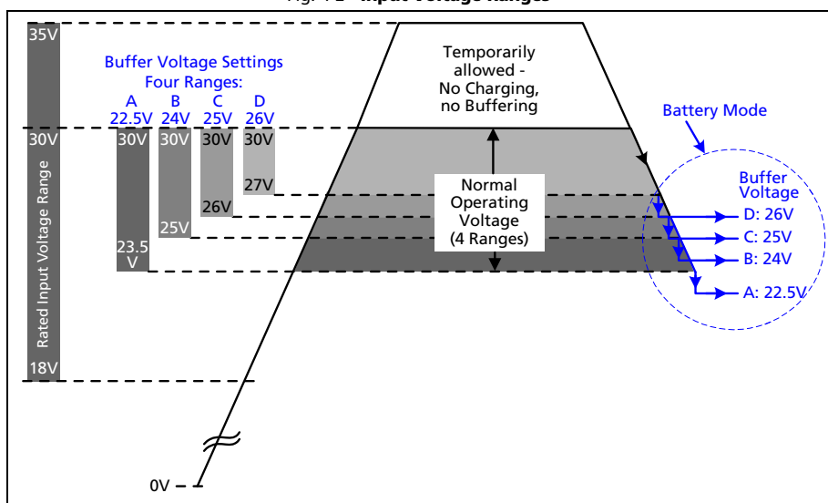
Fig. 4-2 Input Voltage Ranges
