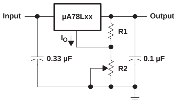
Figure 3. Adjustable-Output Regulator
