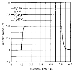
LARGE SIGNAL FEEDFORWARD TRANSIENT RESPONSE
