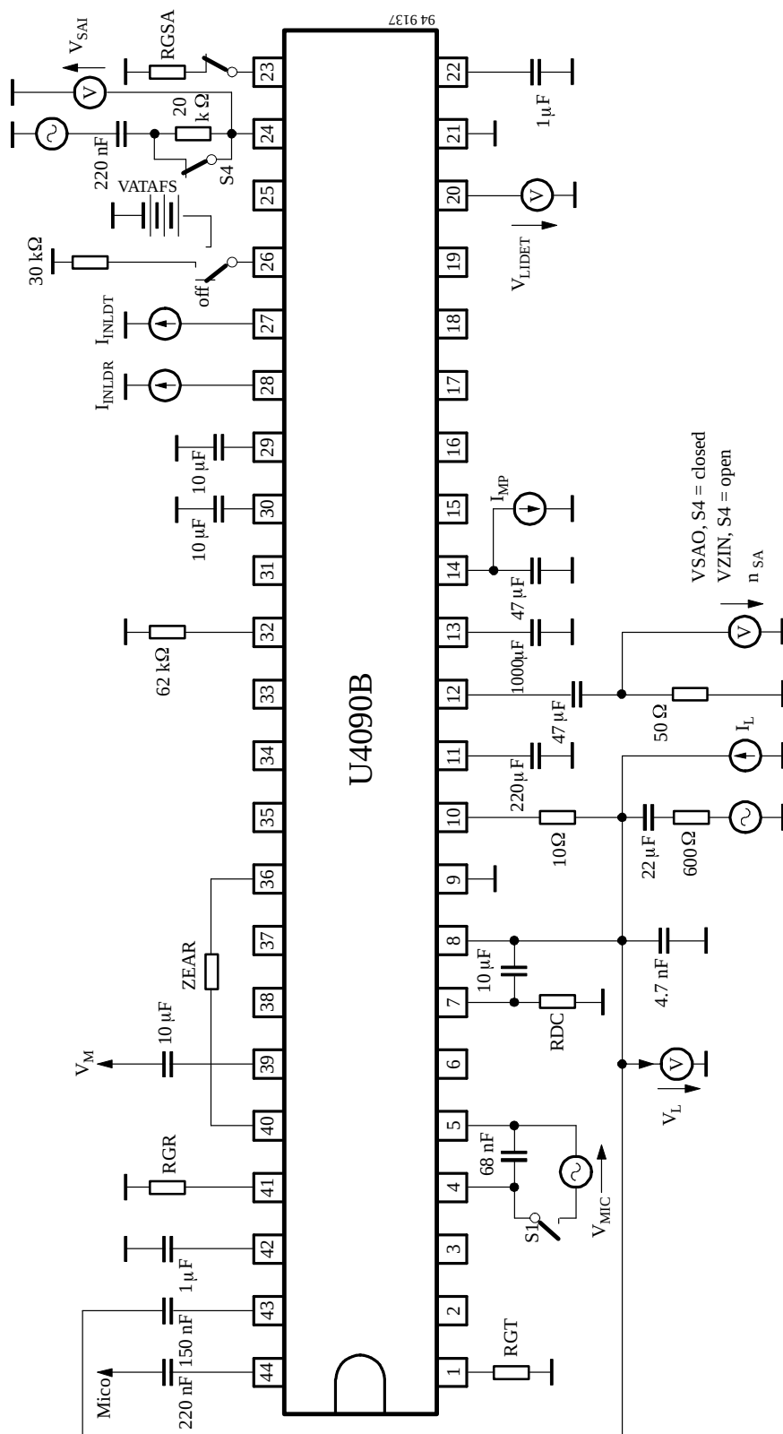
Figure 25. Speaker amplifier
